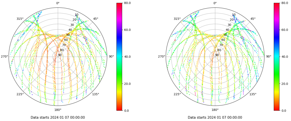
Skyplot for station TAR0. Parameter M1C Data file TAR000ESP_R_2024007.xtr Skyplot for station TAR0. Parameter M2P Data file TAR000ESP_R_2024007.xtr
