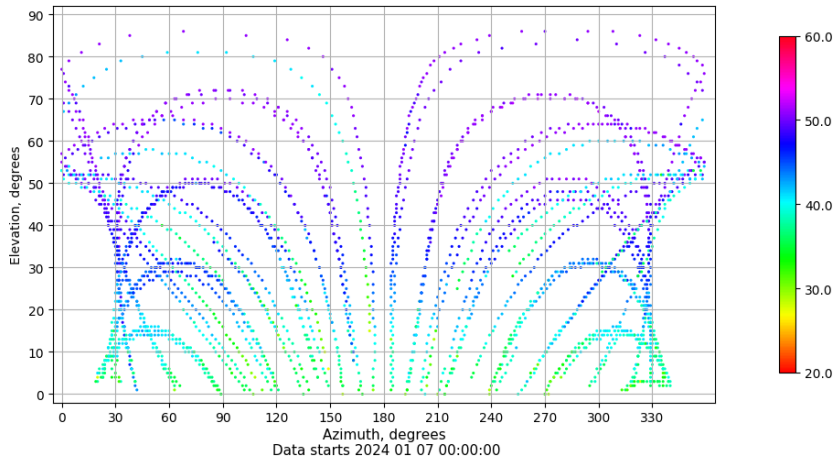
Azimuth-elevation plot for station TAR0. Signal to Noise S1C Data file TAR000ESP_R_2024007.xtr
