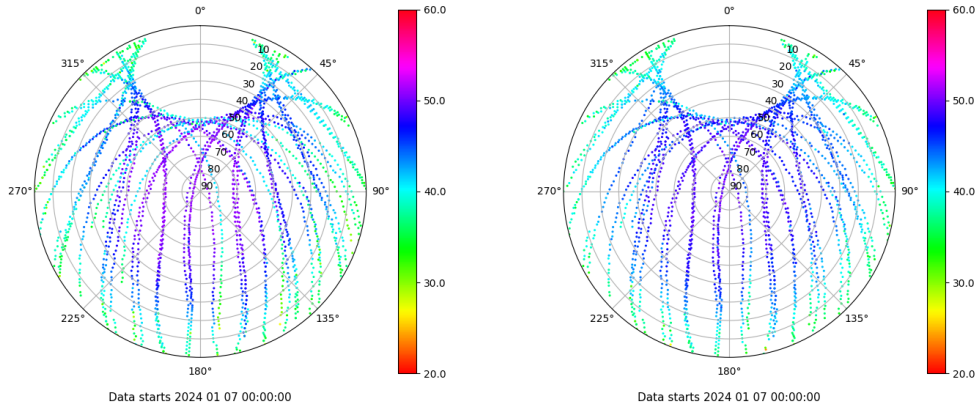
Skyplot for station TAR0. Signal to Noise S1C Data file TAR000ESP_R_2024007.xtr Skyplot for station TAR0. Signal to Noise S2P Data file TAR000ESP_R_2024007.xtr
