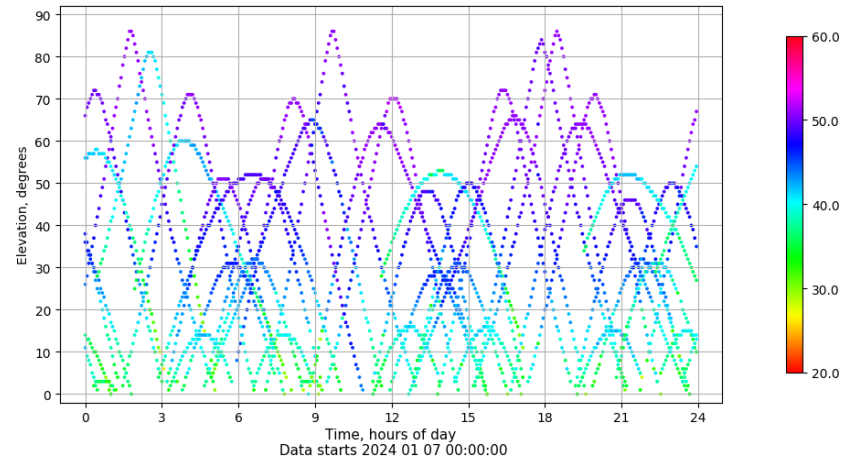
Time-elevation plot for station TAR0. Signal to Noise S1C Data file TAR000ESP_R_2024007.xtr
