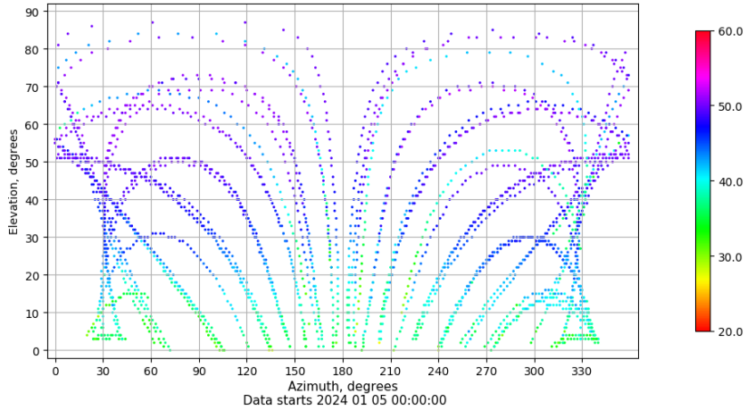
Azimuth-elevation plot for station TAR0. Signal to Noise S1C Data file TAR000ESP_R_2024005.xtr
