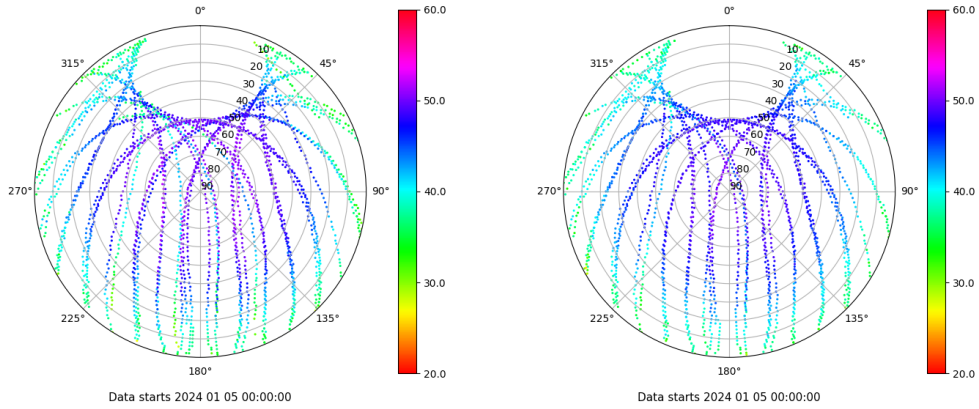
Skyplot for station TAR0. Signal to Noise S1C Data file TAR000ESP_R_2024005.xtr Skyplot for station TAR0. Signal to Noise S2P Data file TAR000ESP_R_2024005.xtr
