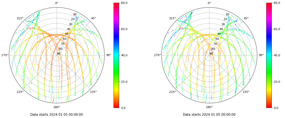
Skyplot for station TAR0. Parameter M1C Data file TAR000ESP_R_2024005.xtr Skyplot for station TAR0. Parameter M2P Data file TAR000ESP_R_2024005.xtr
