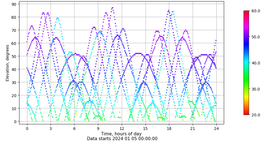
Time-elevation plot for station TAR0. Signal to Noise S1C Data file TAR000ESP_R_2024005.xtr
