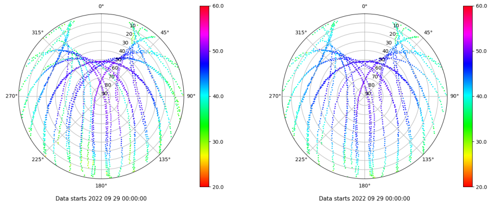
Skyplot for station TAR0. Signal to Noise S1C Data file TAR000ESP_R_2022272.xtr Skyplot for station TAR0. Signal to Noise S2P Data file TAR000ESP_R_2022272.xtr
