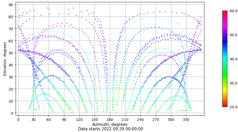
Azimuth-elevation plot for station TAR0. Signal to Noise S1C Data file TAR000ESP_R_2022272.xtr
