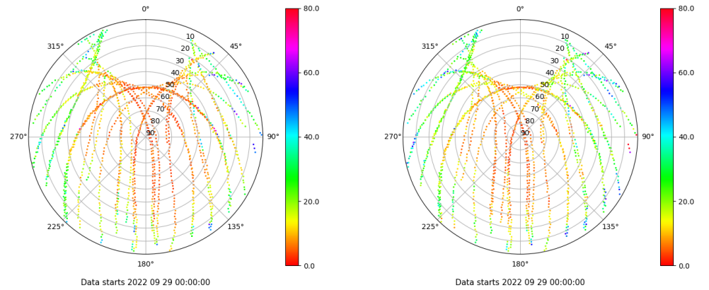
Skyplot for station TAR0. Parameter M1C Data file TAR000ESP_R_2022272.xtr Skyplot for station TAR0. Parameter M2P Data file TAR000ESP_R_2022272.xtr
