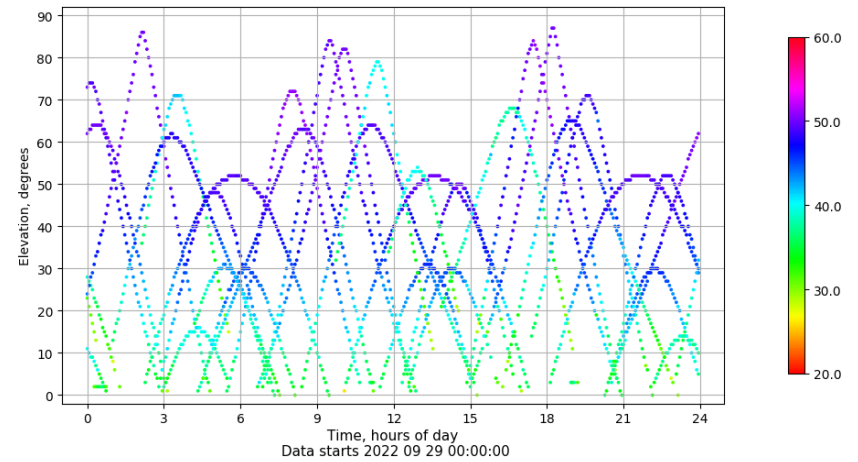
Time-elevation plot for station TAR0. Signal to Noise S1C Data file TAR000ESP_R_2022272.xtr
