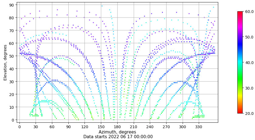
Azimuth-elevation plot for station TAR0. Signal to Noise S1C Data file TAR000ESP_R_2022168.xtr
