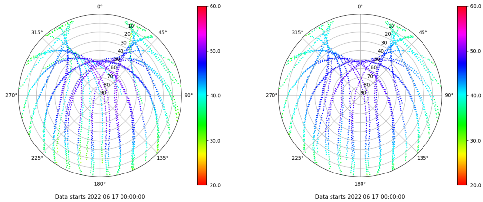
Skyplot for station TAR0. Signal to Noise S1C Data file TAR000ESP_R_2022168.xtr Skyplot for station TAR0. Signal to Noise S2P Data file TAR000ESP_R_2022168.xtr
