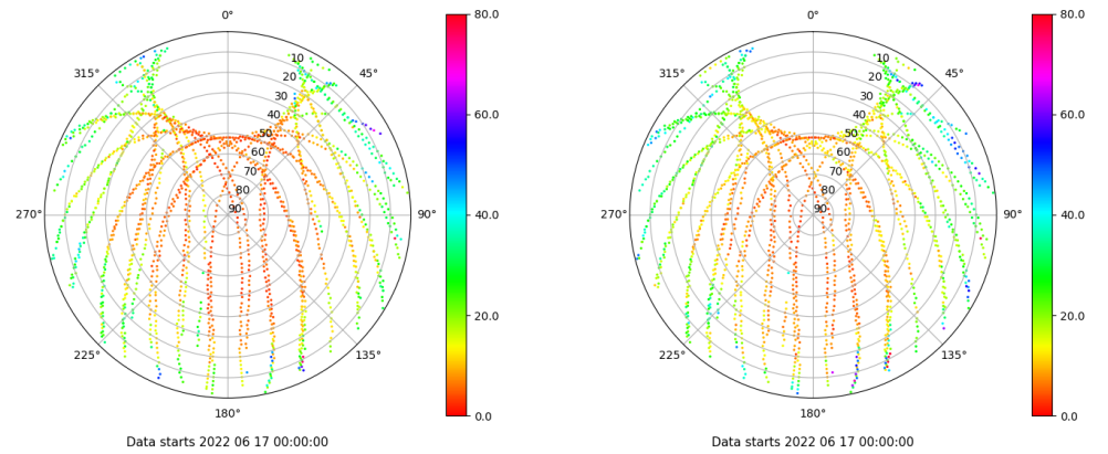
Skyplot for station TAR0. Parameter M1C Data file TAR000ESP_R_2022168.xtr Skyplot for station TAR0. Parameter M2P Data file TAR000ESP_R_2022168.xtr
