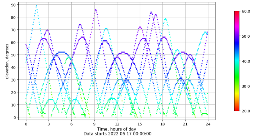
Time-elevation plot for station TAR0. Signal to Noise S1C Data file TAR000ESP_R_2022168.xtr
