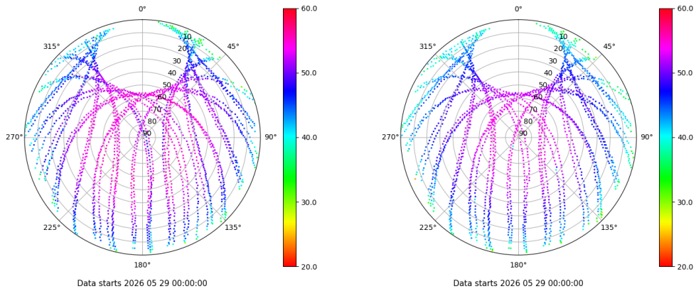
Skyplot for station TALV. Signal to Noise S1C Data file TALV00ESP_R_2026149.xtr Skyplot for station TALV. Signal to Noise S2P Data file TALV00ESP_R_2026149.xtr
