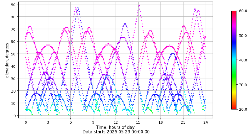
Time-elevation plot for station TALV. Signal to Noise S1C Data file TALV00ESP_R_2026149.xtr
