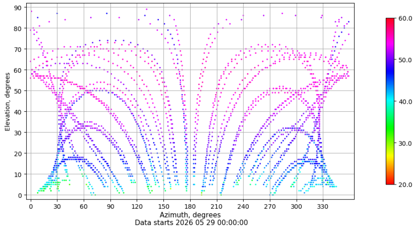
Azimuth-elevation plot for station TALV. Signal to Noise S1C Data file TALV00ESP_R_2026149.xtr
