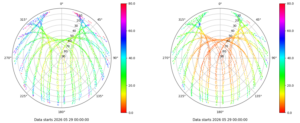
Skyplot for station TALV. Parameter M1C Data file TALV00ESP_R_2026149.xtr Skyplot for station TALV. Parameter M2P Data file TALV00ESP_R_2026149.xtr
