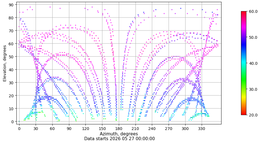
Azimuth-elevation plot for station TALV. Signal to Noise S1C Data file TALV00ESP_R_2026147.xtr
