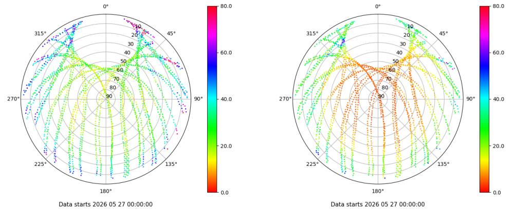
Skyplot for station TALV. Parameter M1C Data file TALV00ESP_R_2026147.xtr Skyplot for station TALV. Parameter M2P Data file TALV00ESP_R_2026147.xtr
