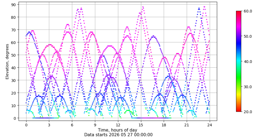
Time-elevation plot for station TALV. Signal to Noise S1C Data file TALV00ESP_R_2026147.xtr
