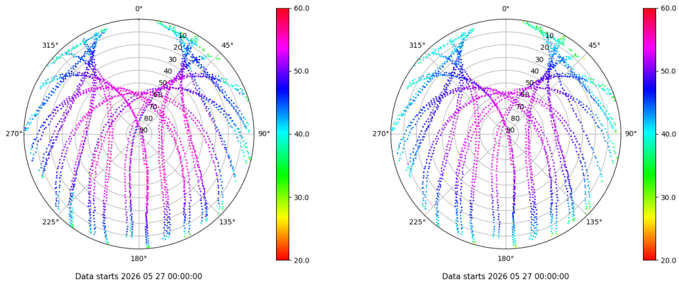
Skyplot for station TALV. Signal to Noise S1C Data file TALV00ESP_R_2026147.xtr Skyplot for station TALV. Signal to Noise S2P Data file TALV00ESP_R_2026147.xtr
