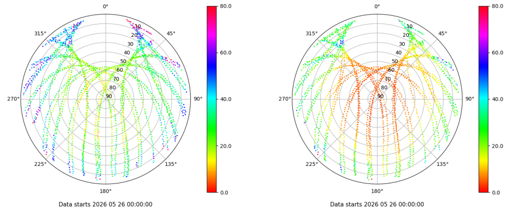
Skyplot for station TALV. Parameter M1C Data file TALV00ESP_R_2026146.xtr Skyplot for station TALV. Parameter M2P Data file TALV00ESP_R_2026146.xtr
