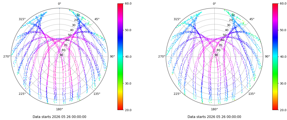
Skyplot for station TALV. Signal to Noise S1C Data file TALV00ESP_R_2026146.xtr Skyplot for station TALV. Signal to Noise S2P Data file TALV00ESP_R_2026146.xtr
