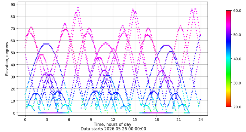
Time-elevation plot for station TALV. Signal to Noise S1C Data file TALV00ESP_R_2026146.xtr
