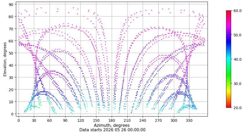
Azimuth-elevation plot for station TALV. Signal to Noise S1C Data file TALV00ESP_R_2026146.xtr
