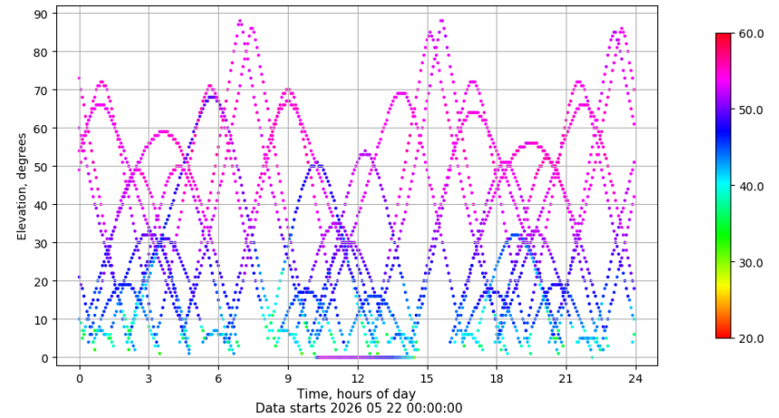
Time-elevation plot for station TALV. Signal to Noise S1C Data file TALV00ESP_R_2026142.xtr
