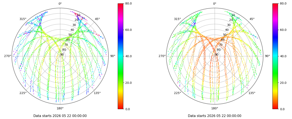
Skyplot for station TALV. Parameter M1C Data file TALV00ESP_R_2026142.xtr Skyplot for station TALV. Parameter M2P Data file TALV00ESP_R_2026142.xtr
