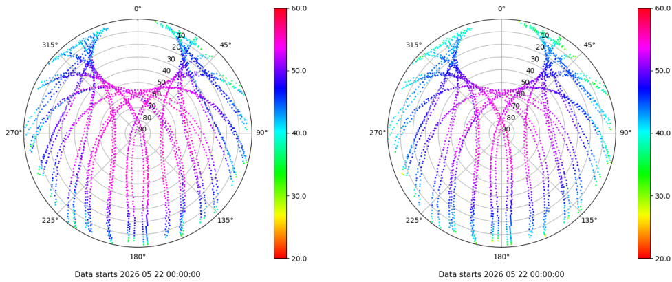
Skyplot for station TALV. Signal to Noise S1C Data file TALV00ESP_R_2026142.xtr Skyplot for station TALV. Signal to Noise S2P Data file TALV00ESP_R_2026142.xtr
