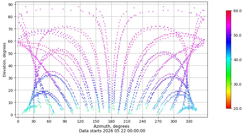
Azimuth-elevation plot for station TALV. Signal to Noise S1C Data file TALV00ESP_R_2026142.xtr
