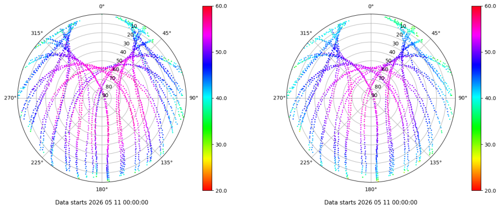
Skyplot for station TALV. Signal to Noise S1C Data file TALV00ESP_R_2026131.xtr Skyplot for station TALV. Signal to Noise S2P Data file TALV00ESP_R_2026131.xtr
