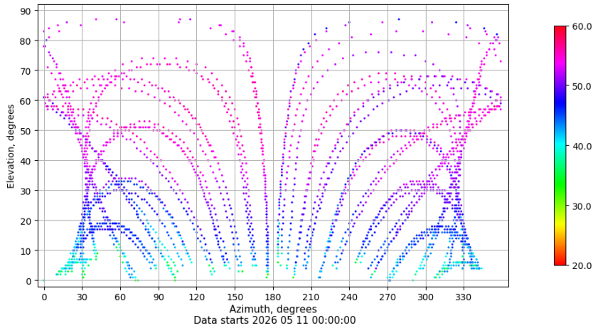
Azimuth-elevation plot for station TALV. Signal to Noise S1C Data file TALV00ESP_R_2026131.xtr
