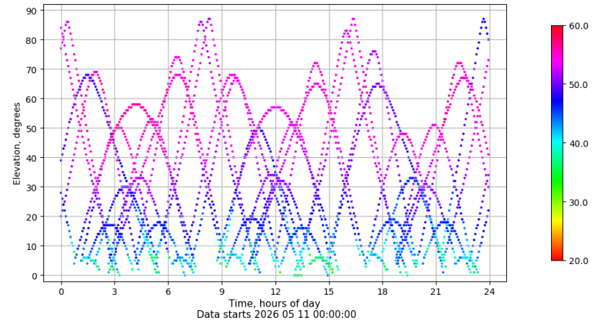
Time-elevation plot for station TALV. Signal to Noise S1C Data file TALV00ESP_R_2026131.xtr
