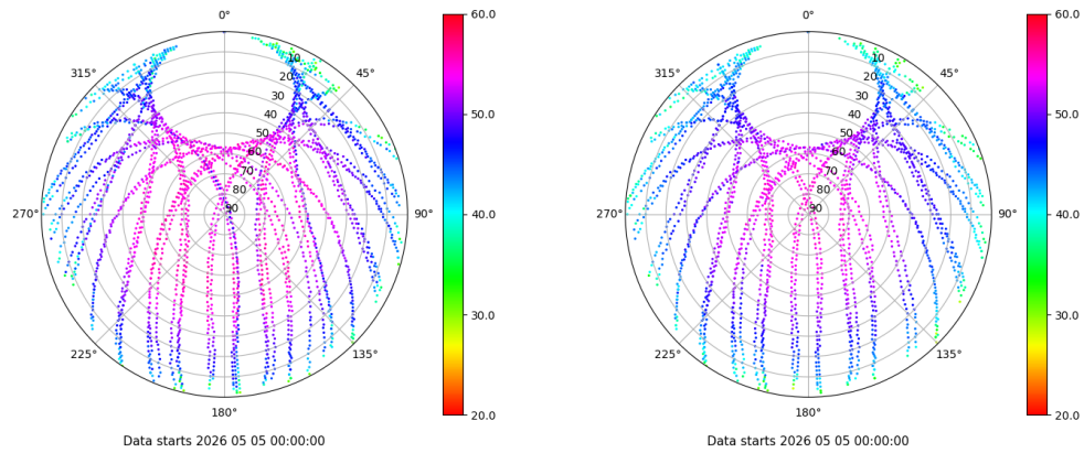
Skyplot for station TALV. Signal to Noise S1C Data file TALV00ESP_R_2026125.xtr Skyplot for station TALV. Signal to Noise S2P Data file TALV00ESP_R_2026125.xtr
