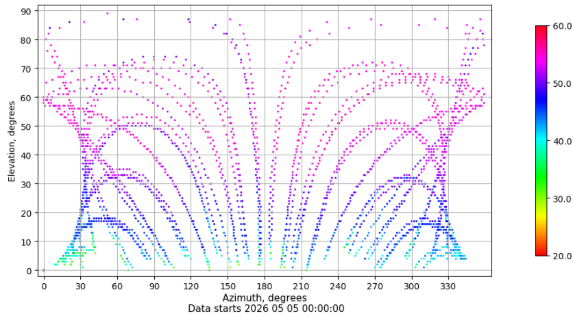
Azimuth-elevation plot for station TALV. Signal to Noise S1C Data file TALV00ESP_R_2026125.xtr
