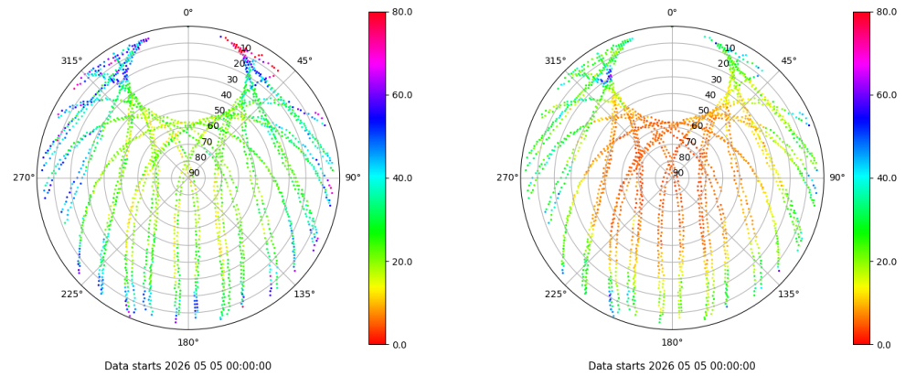
Skyplot for station TALV. Parameter M1C Data file TALV00ESP_R_2026125.xtr Skyplot for station TALV. Parameter M2P Data file TALV00ESP_R_2026125.xtr
