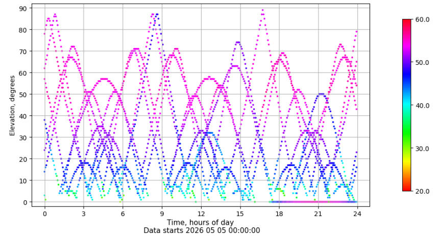
Time-elevation plot for station TALV. Signal to Noise S1C Data file TALV00ESP_R_2026125.xtr
