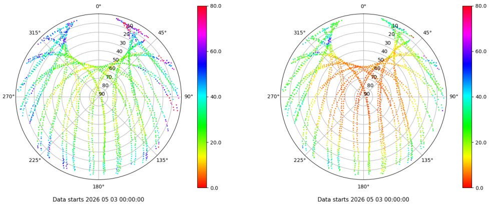
Skyplot for station TALV. Parameter M1C Data file TALV00ESP_R_2026123.xtr Skyplot for station TALV. Parameter M2P Data file TALV00ESP_R_2026123.xtr
