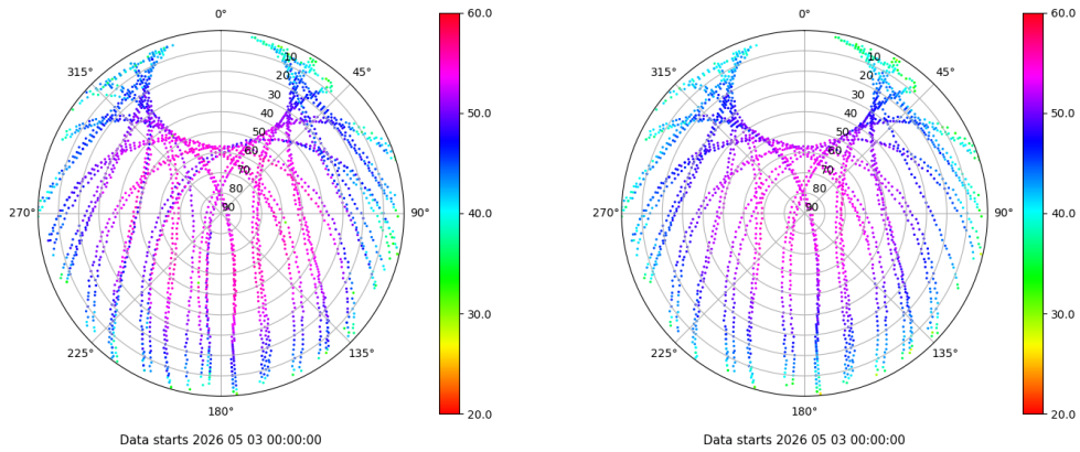
Skyplot for station TALV. Signal to Noise S1C Data file TALV00ESP_R_2026123.xtr Skyplot for station TALV. Signal to Noise S2P Data file TALV00ESP_R_2026123.xtr
