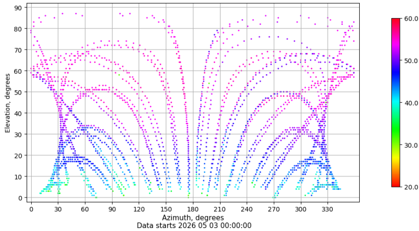
Azimuth-elevation plot for station TALV. Signal to Noise S1C Data file TALV00ESP_R_2026123.xtr
