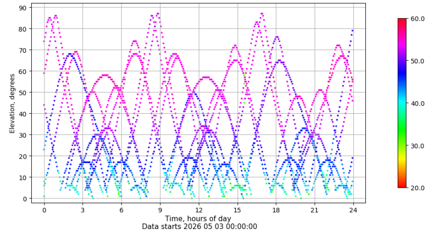
Time-elevation plot for station TALV. Signal to Noise S1C Data file TALV00ESP_R_2026123.xtr
