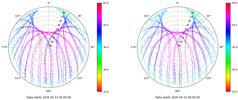
Skyplot for station TALV. Signal to Noise S1C Data file TALV00ESP_R_2026113.xtr Skyplot for station TALV. Signal to Noise S2P Data file TALV00ESP_R_2026113.xtr
