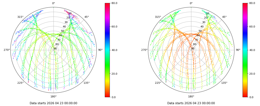
Skyplot for station TALV. Parameter M1C Data file TALV00ESP_R_2026113.xtr Skyplot for station TALV. Parameter M2P Data file TALV00ESP_R_2026113.xtr
