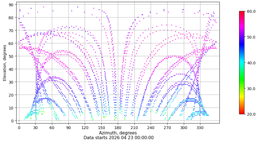
Azimuth-elevation plot for station TALV. Signal to Noise S1C Data file TALV00ESP_R_2026113.xtr
