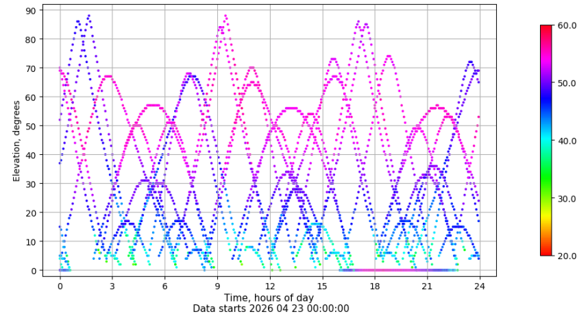
Time-elevation plot for station TALV. Signal to Noise S1C Data file TALV00ESP_R_2026113.xtr
