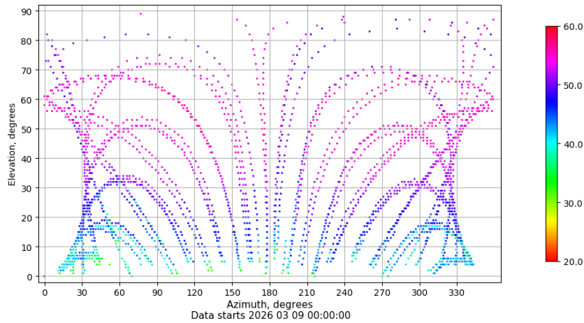
Azimuth-elevation plot for station TALV. Signal to Noise S1C Data file TALV00ESP_R_2026068.xtr
