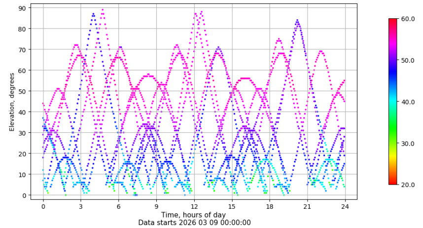
Time-elevation plot for station TALV. Signal to Noise S1C Data file TALV00ESP_R_2026068.xtr
