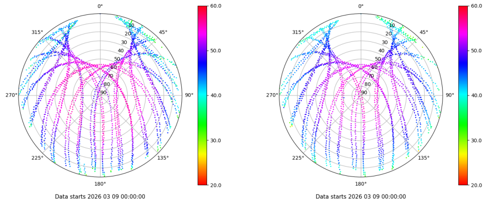
Skyplot for station TALV. Signal to Noise S1C Data file TALV00ESP_R_2026068.xtr Skyplot for station TALV. Signal to Noise S2P Data file TALV00ESP_R_2026068.xtr
