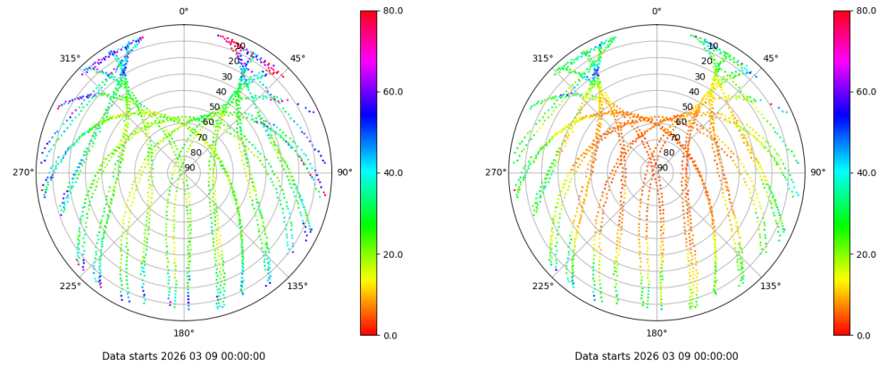
Skyplot for station TALV. Parameter M1C Data file TALV00ESP_R_2026068.xtr Skyplot for station TALV. Parameter M2P Data file TALV00ESP_R_2026068.xtr
