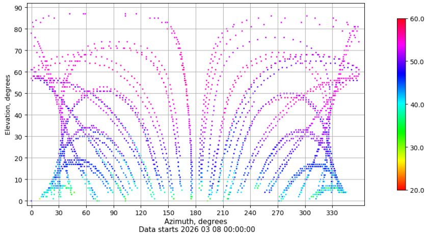
Azimuth-elevation plot for station TALV. Signal to Noise S1C Data file TALV00ESP_R_2026067.xtr
