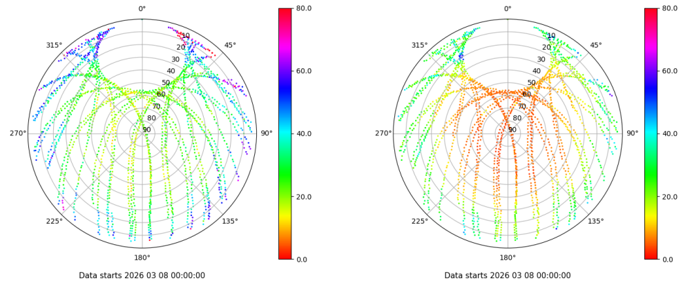
Skyplot for station TALV. Parameter M1C Data file TALV00ESP_R_2026067.xtr Skyplot for station TALV. Parameter M2P Data file TALV00ESP_R_2026067.xtr
