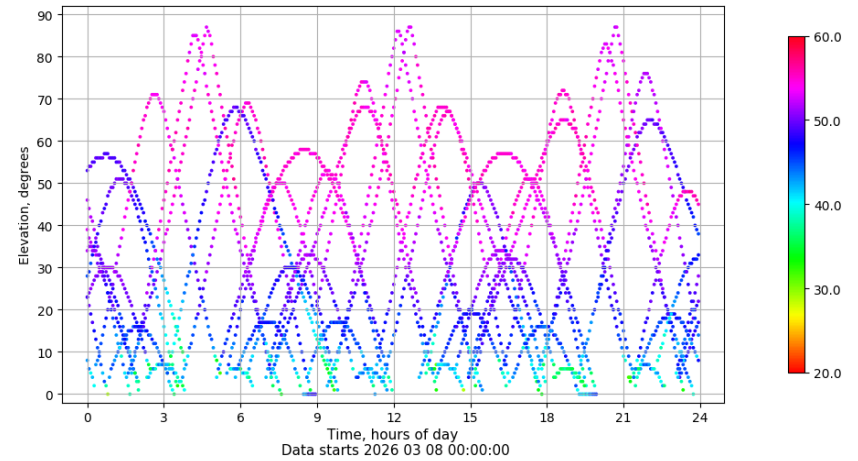
Time-elevation plot for station TALV. Signal to Noise S1C Data file TALV00ESP_R_2026067.xtr
