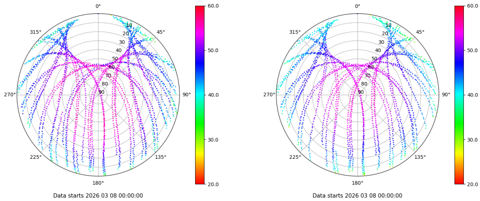
Skyplot for station TALV. Signal to Noise S1C Data file TALV00ESP_R_2026067.xtr Skyplot for station TALV. Signal to Noise S2P Data file TALV00ESP_R_2026067.xtr
