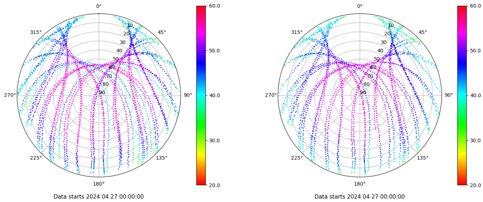
Skyplot for station TALV. Signal to Noise S1C Data file TALV00ESP_R_2024118.xtr Skyplot for station TALV. Signal to Noise S2P Data file TALV00ESP_R_2024118.xtr
