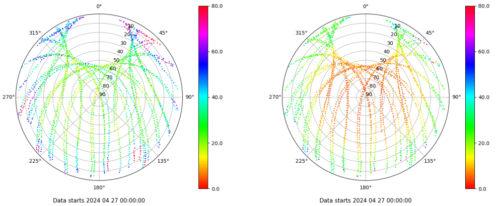
Skyplot for station TALV. Parameter M1C Data file TALV00ESP_R_2024118.xtr Skyplot for station TALV. Parameter M2P Data file TALV00ESP_R_2024118.xtr
