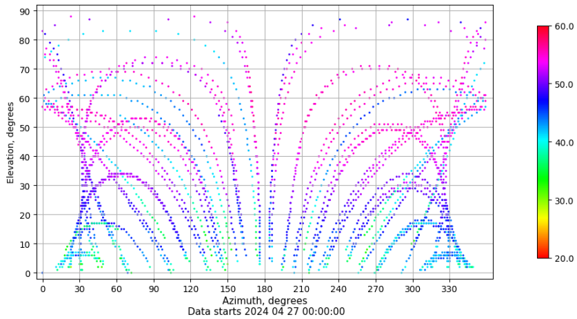
Azimuth-elevation plot for station TALV. Signal to Noise S1C Data file TALV00ESP_R_2024118.xtr
