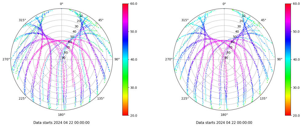
Skyplot for station TALV. Signal to Noise S1C Data file TALV00ESP_R_2024113.xtr Skyplot for station TALV. Signal to Noise S2P Data file TALV00ESP_R_2024113.xtr
