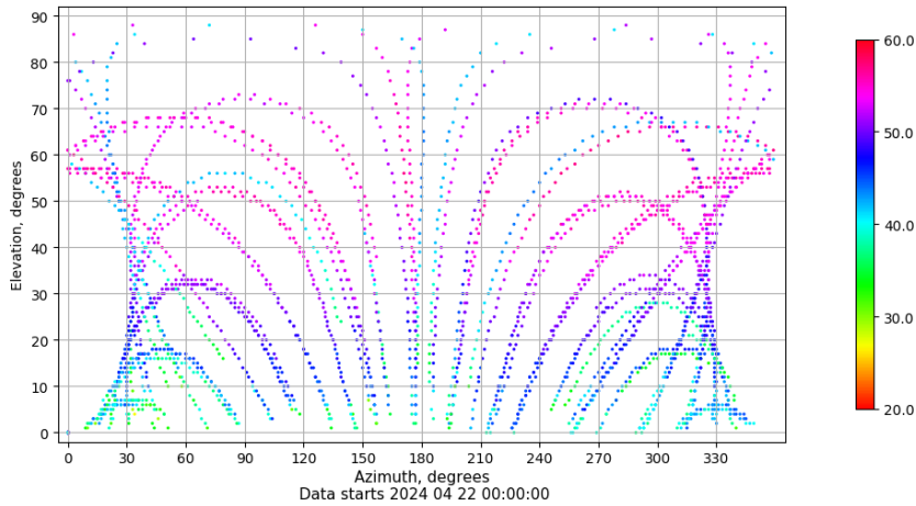
Azimuth-elevation plot for station TALV. Signal to Noise S1C Data file TALV00ESP_R_2024113.xtr
