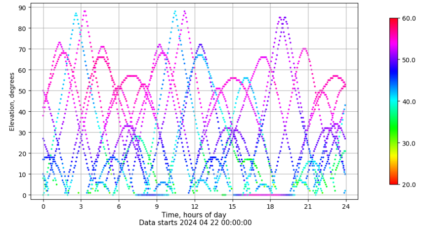
Time-elevation plot for station TALV. Signal to Noise S1C Data file TALV00ESP_R_2024113.xtr
