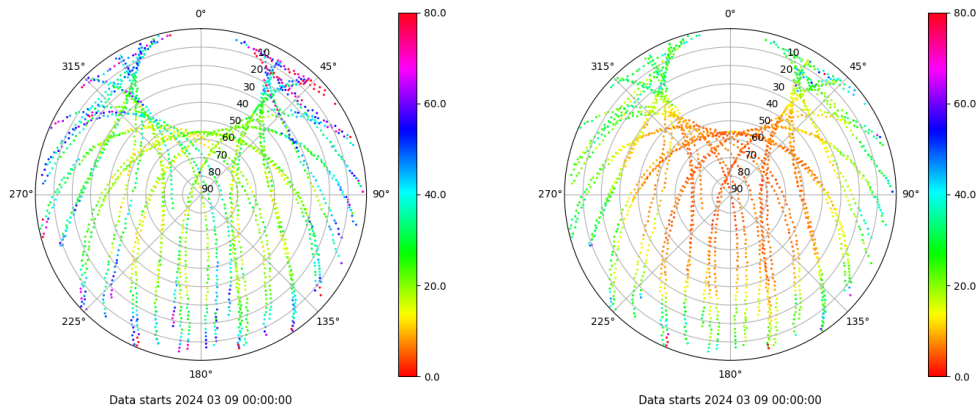
Skyplot for station TALV. Parameter M1C Data file TALV00ESP_R_2024069.xtr Skyplot for station TALV. Parameter M2P Data file TALV00ESP_R_2024069.xtr
