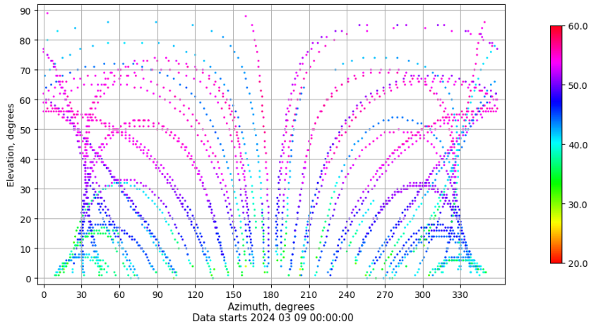
Azimuth-elevation plot for station TALV. Signal to Noise S1C Data file TALV00ESP_R_2024069.xtr
