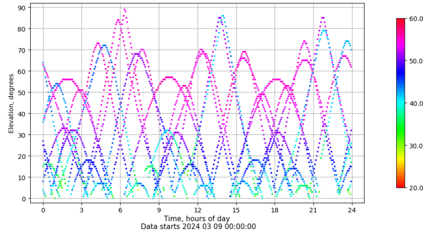
Time-elevation plot for station TALV. Signal to Noise S1C Data file TALV00ESP_R_2024069.xtr
