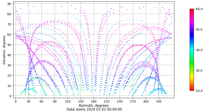
Azimuth-elevation plot for station TALV. Signal to Noise S1C Data file TALV00ESP_R_2024062.xtr
