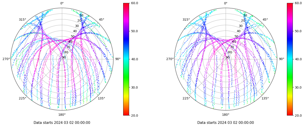
Skyplot for station TALV. Signal to Noise S1C Data file TALV00ESP_R_2024062.xtr Skyplot for station TALV. Signal to Noise S2P Data file TALV00ESP_R_2024062.xtr
