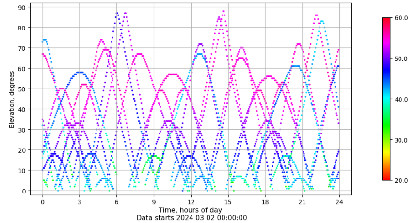
Time-elevation plot for station TALV. Signal to Noise S1C Data file TALV00ESP_R_2024062.xtr
