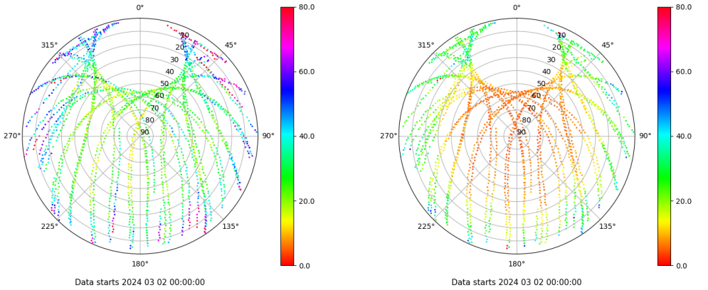
Skyplot for station TALV. Parameter M1C Data file TALV00ESP_R_2024062.xtr Skyplot for station TALV. Parameter M2P Data file TALV00ESP_R_2024062.xtr
