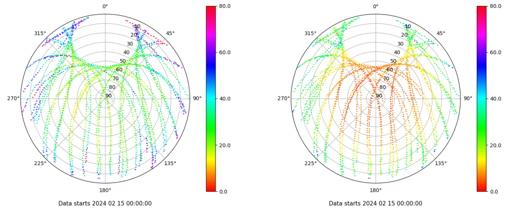
Skyplot for station TALV. Parameter M1C Data file TALV00ESP_R_2024046.xtr Skyplot for station TALV. Parameter M2P Data file TALV00ESP_R_2024046.xtr
