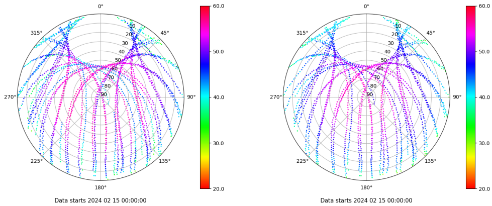
Skyplot for station TALV. Signal to Noise S1C Data file TALV00ESP_R_2024046.xtr Skyplot for station TALV. Signal to Noise S2P Data file TALV00ESP_R_2024046.xtr
