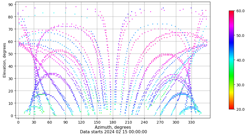
Azimuth-elevation plot for station TALV. Signal to Noise S1C Data file TALV00ESP_R_2024046.xtr
