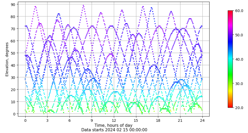
Time-elevation plot for station TALV. Signal to Noise S1C Data file TALV00ESP_R_2024046.xtr
