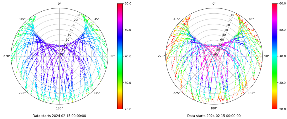
Skyplot for station TALV. Signal to Noise S1C Data file TALV00ESP_R_2024046.xtr Skyplot for station TALV. Signal to Noise S2W Data file TALV00ESP_R_2024046.xtr
