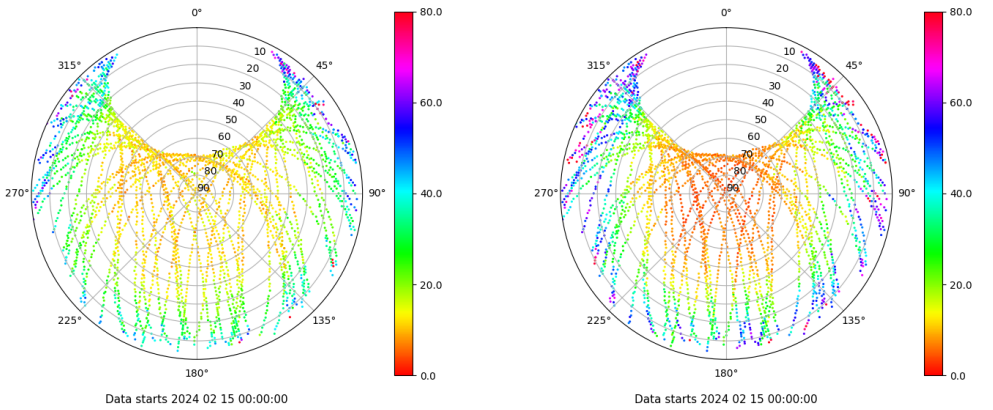
Skyplot for station TALV. Parameter M1C Data file TALV00ESP_R_2024046.xtr Skyplot for station TALV. Parameter M2W Data file TALV00ESP_R_2024046.xtr
