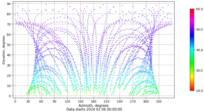
Azimuth-elevation plot for station TALV. Signal to Noise S1C Data file TALV00ESP_R_2024037.xtr
