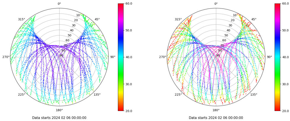
Skyplot for station TALV. Signal to Noise S1C Data file TALV00ESP_R_2024037.xtr Skyplot for station TALV. Signal to Noise S2W Data file TALV00ESP_R_2024037.xtr
