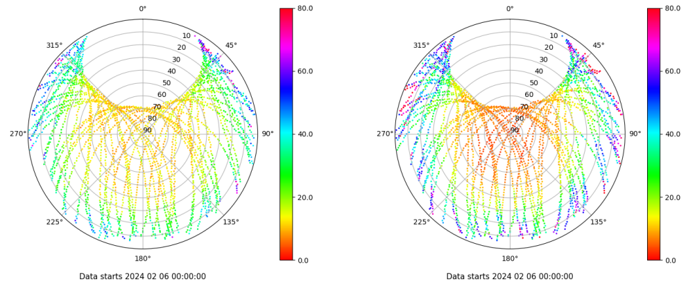
Skyplot for station TALV. Parameter M1C Data file TALV00ESP_R_2024037.xtr Skyplot for station TALV. Parameter M2W Data file TALV00ESP_R_2024037.xtr
