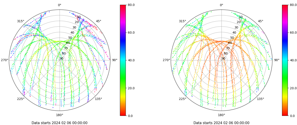
Skyplot for station TALV. Parameter M1C Data file TALV00ESP_R_2024037.xtr Skyplot for station TALV. Parameter M2P Data file TALV00ESP_R_2024037.xtr
