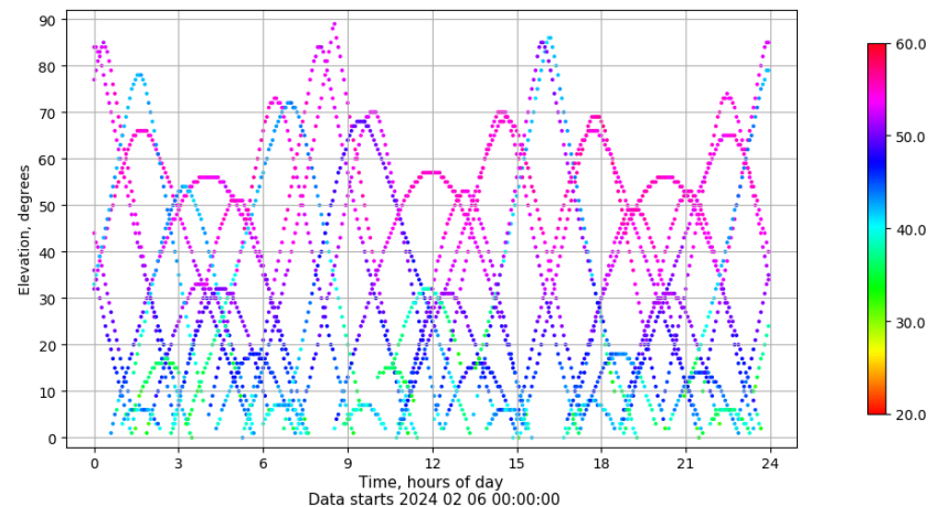
Time-elevation plot for station TALV. Signal to Noise S1C Data file TALV00ESP_R_2024037.xtr
