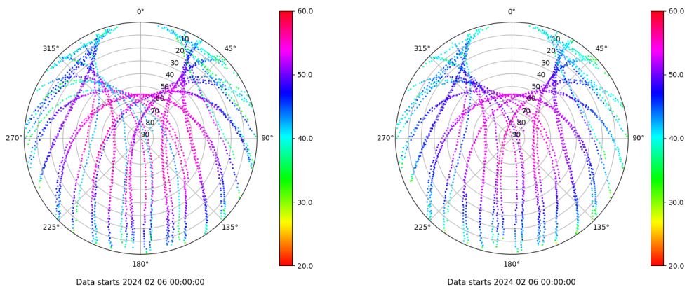
Skyplot for station TALV. Signal to Noise S1C Data file TALV00ESP_R_2024037.xtr Skyplot for station TALV. Signal to Noise S2P Data file TALV00ESP_R_2024037.xtr
