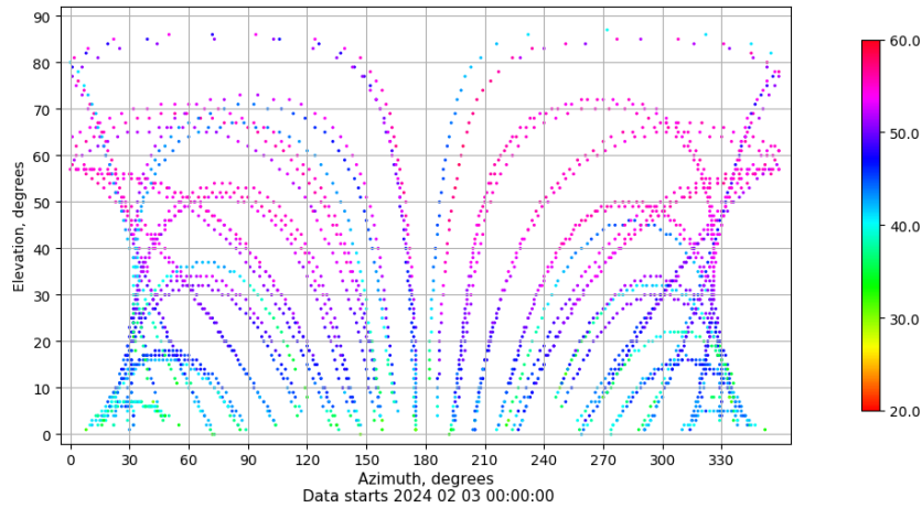
Azimuth-elevation plot for station TALV. Signal to Noise S1C Data file TALV00ESP_R_2024034.xtr
