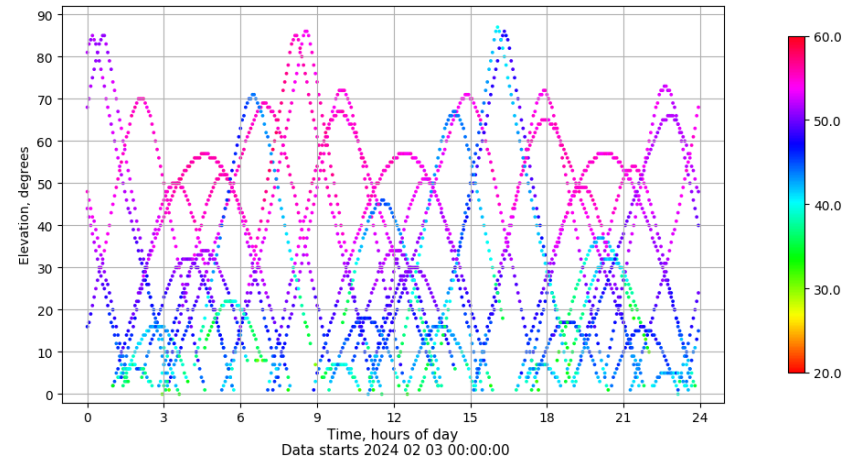
Time-elevation plot for station TALV. Signal to Noise S1C Data file TALV00ESP_R_2024034.xtr
