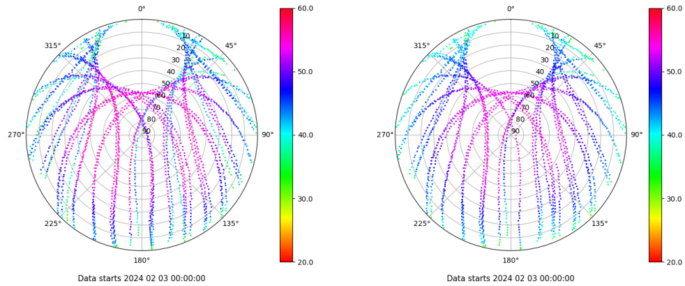
Skyplot for station TALV. Signal to Noise S1C Data file TALV00ESP_R_2024034.xtr Skyplot for station TALV. Signal to Noise S2P Data file TALV00ESP_R_2024034.xtr
