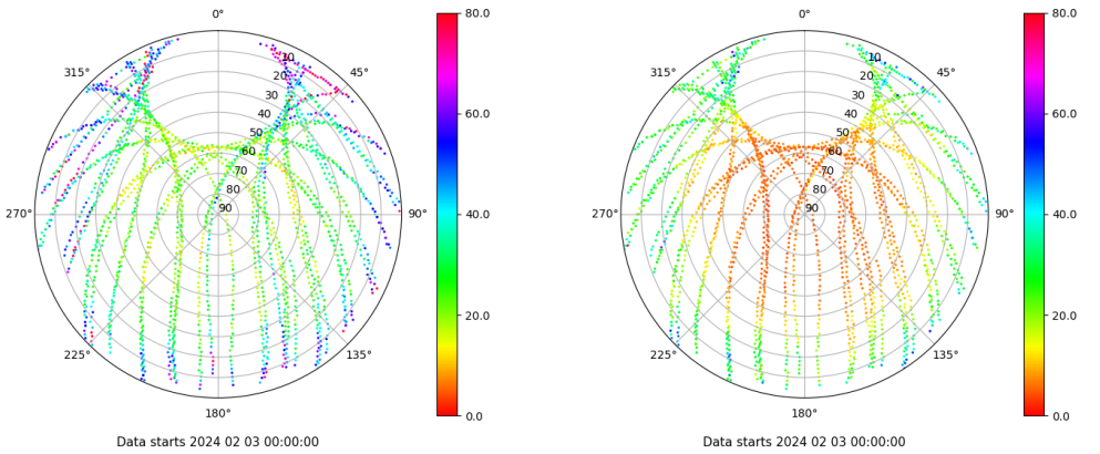
Skyplot for station TALV. Parameter M1C Data file TALV00ESP_R_2024034.xtr Skyplot for station TALV. Parameter M2P Data file TALV00ESP_R_2024034.xtr
