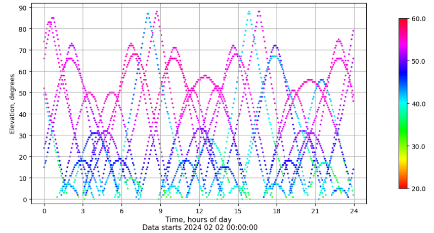
Time-elevation plot for station TALV. Signal to Noise S1C Data file TALV00ESP_R_2024033.xtr
