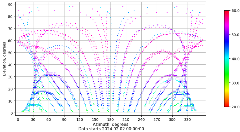
Azimuth-elevation plot for station TALV. Signal to Noise S1C Data file TALV00ESP_R_2024033.xtr
