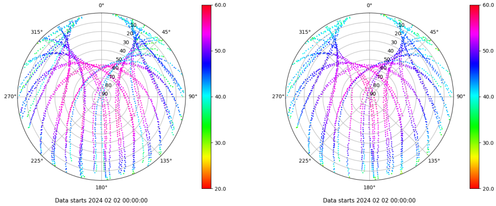
Skyplot for station TALV. Signal to Noise S1C Data file TALV00ESP_R_2024033.xtr Skyplot for station TALV. Signal to Noise S2P Data file TALV00ESP_R_2024033.xtr
