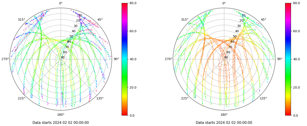
Skyplot for station TALV. Parameter M1C Data file TALV00ESP_R_2024033.xtr Skyplot for station TALV. Parameter M2P Data file TALV00ESP_R_2024033.xtr
