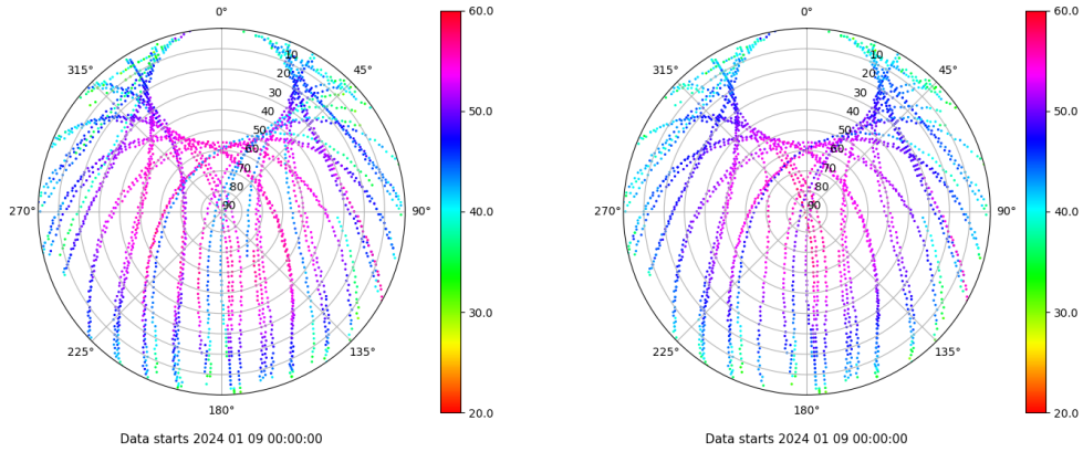
Skyplot for station TALV. Signal to Noise S1C Data file TALV00ESP_R_2024009.xtr Skyplot for station TALV. Signal to Noise S2P Data file TALV00ESP_R_2024009.xtr
