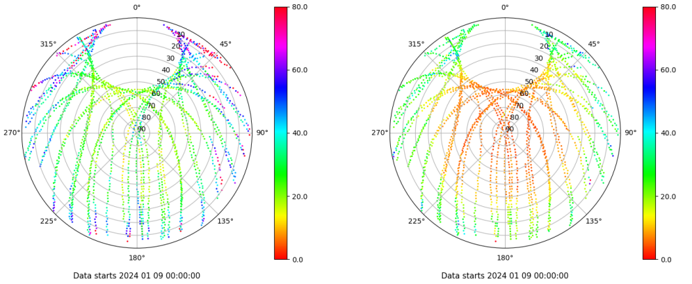
Skyplot for station TALV. Parameter M1C Data file TALV00ESP_R_2024009.xtr Skyplot for station TALV. Parameter M2P Data file TALV00ESP_R_2024009.xtr
