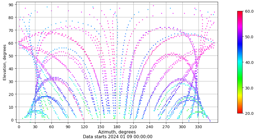
Azimuth-elevation plot for station TALV. Signal to Noise S1C Data file TALV00ESP_R_2024009.xtr
