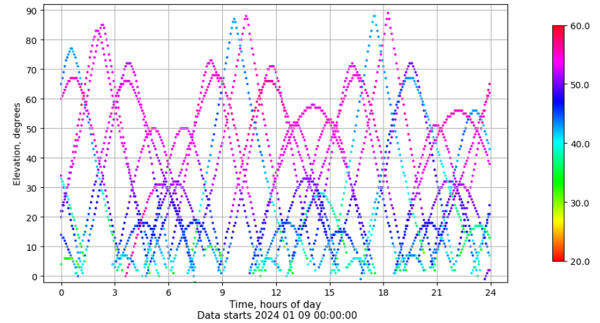
Time-elevation plot for station TALV. Signal to Noise S1C Data file TALV00ESP_R_2024009.xtr
