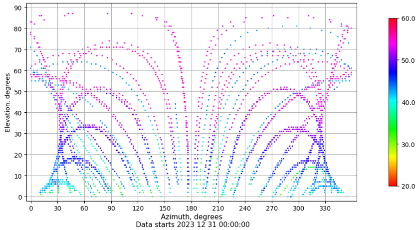
Azimuth-elevation plot for station TALV. Signal to Noise S1C Data file TALV00ESP_R_2023365.xtr
