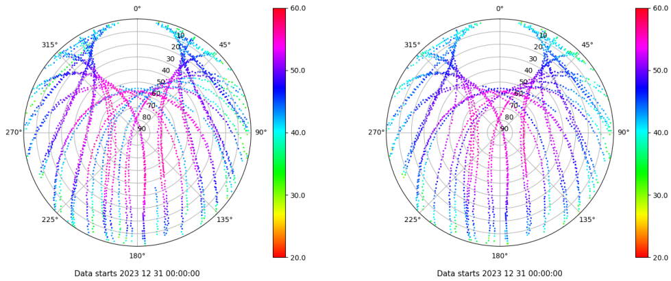
Skyplot for station TALV. Signal to Noise S1C Data file TALV00ESP_R_2023365.xtr Skyplot for station TALV. Signal to Noise S2P Data file TALV00ESP_R_2023365.xtr
