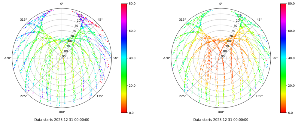
Skyplot for station TALV. Parameter M1C Data file TALV00ESP_R_2023365.xtr Skyplot for station TALV. Parameter M2P Data file TALV00ESP_R_2023365.xtr
