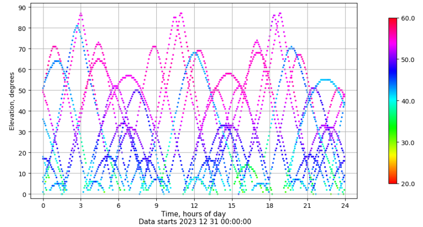
Time-elevation plot for station TALV. Signal to Noise S1C Data file TALV00ESP_R_2023365.xtr
