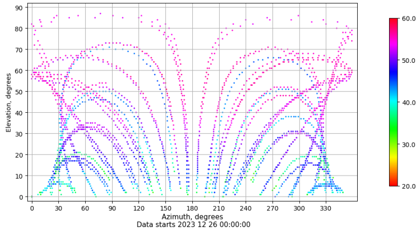
Azimuth-elevation plot for station TALV. Signal to Noise S1C Data file TALV00ESP_R_2023360.xtr
