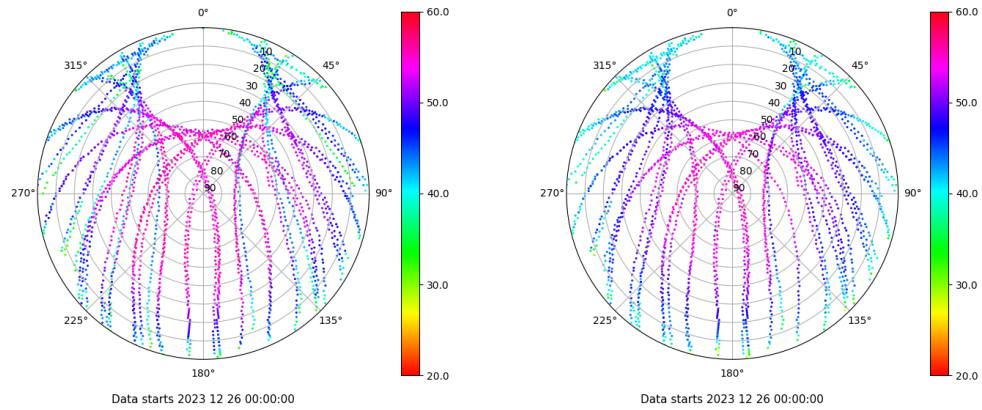
Skyplot for station TALV. Signal to Noise S1C Data file TALV00ESP_R_2023360.xtr Skyplot for station TALV. Signal to Noise S2P Data file TALV00ESP_R_2023360.xtr
