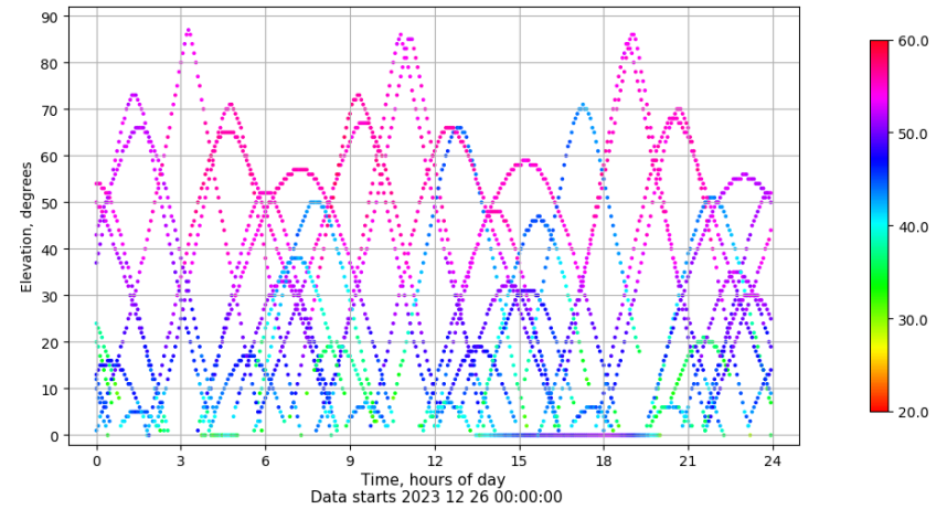
Time-elevation plot for station TALV. Signal to Noise S1C Data file TALV00ESP_R_2023360.xtr
