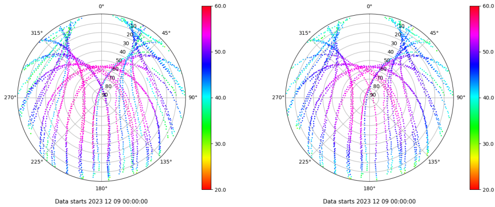
Skyplot for station TALV. Signal to Noise S1C Data file TALV00ESP_R_2023343.xtr Skyplot for station TALV. Signal to Noise S2P Data file TALV00ESP_R_2023343.xtr
