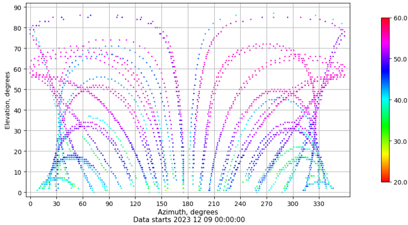
Azimuth-elevation plot for station TALV. Signal to Noise S1C Data file TALV00ESP_R_2023343.xtr
