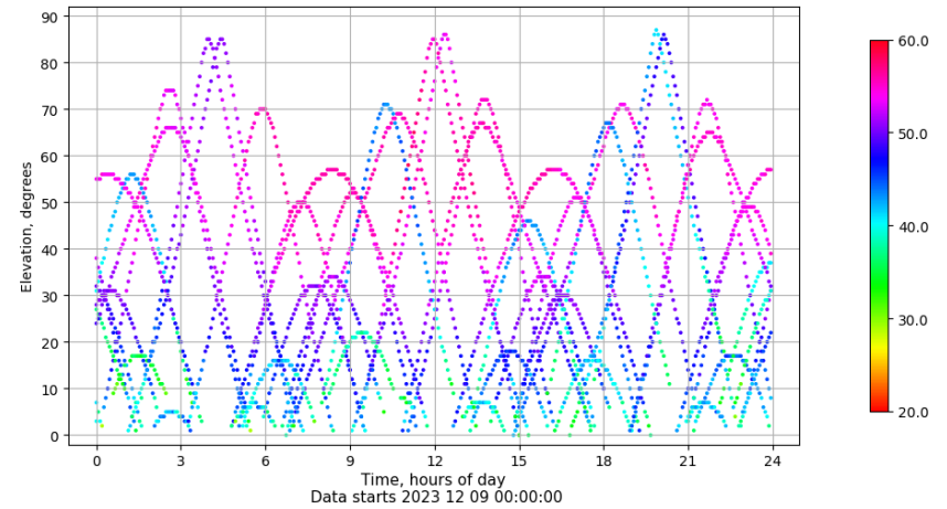
Time-elevation plot for station TALV. Signal to Noise S1C Data file TALV00ESP_R_2023343.xtr
