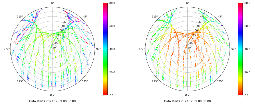
Skyplot for station TALV. Parameter M1C Data file TALV00ESP_R_2023343.xtr Skyplot for station TALV. Parameter M2P Data file TALV00ESP_R_2023343.xtr
