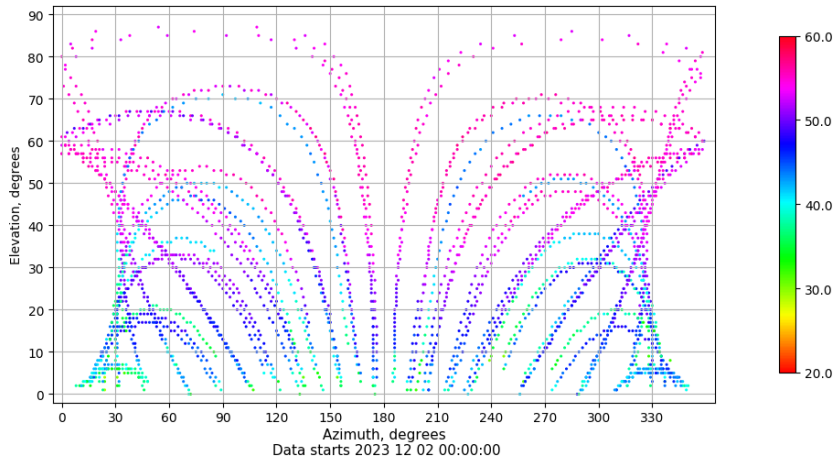
Azimuth-elevation plot for station TALV. Signal to Noise S1C Data file TALV00ESP_R_2023336.xtr
