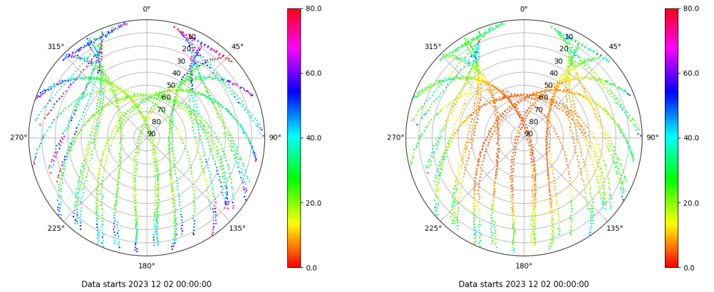
Skyplot for station TALV. Parameter M1C Data file TALV00ESP_R_2023336.xtr Skyplot for station TALV. Parameter M2P Data file TALV00ESP_R_2023336.xtr
