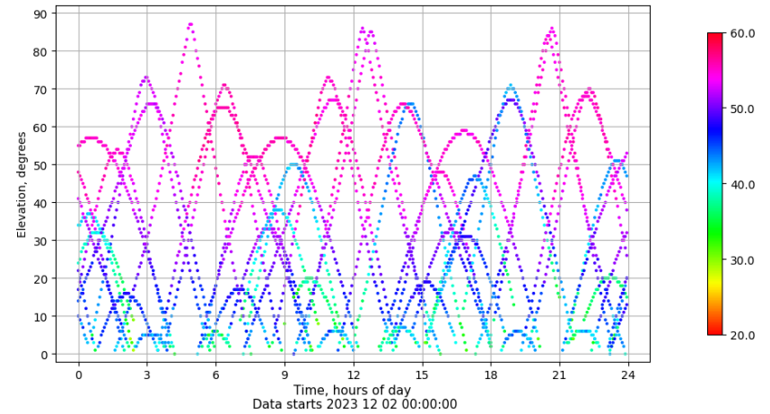
Time-elevation plot for station TALV. Signal to Noise S1C Data file TALV00ESP_R_2023336.xtr
