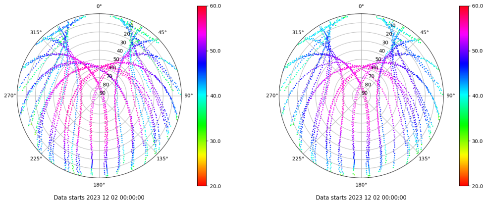
Skyplot for station TALV. Signal to Noise S1C Data file TALV00ESP_R_2023336.xtr Skyplot for station TALV. Signal to Noise S2P Data file TALV00ESP_R_2023336.xtr
