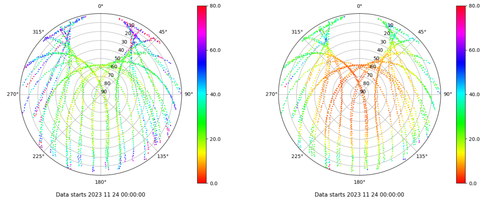
Skyplot for station TALV. Parameter M1C Data file TALV00ESP_R_2023328.xtr Skyplot for station TALV. Parameter M2P Data file TALV00ESP_R_2023328.xtr
