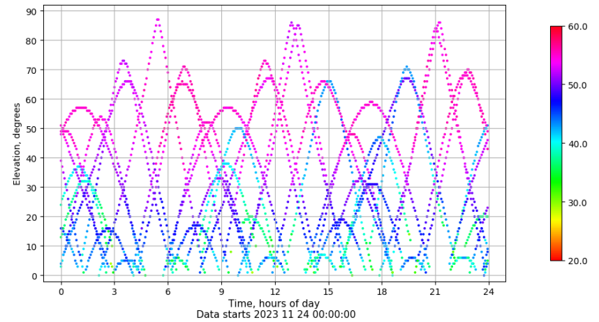
Time-elevation plot for station TALV. Signal to Noise S1C Data file TALV00ESP_R_2023328.xtr
