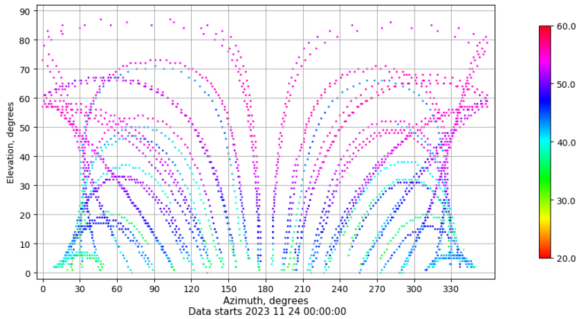
Azimuth-elevation plot for station TALV. Signal to Noise S1C Data file TALV00ESP_R_2023328.xtr
