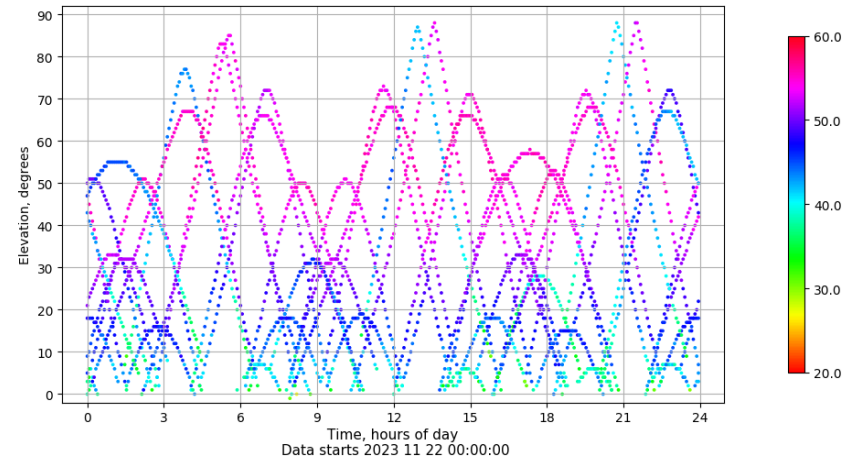
Time-elevation plot for station TALV. Signal to Noise S1C Data file TALV00ESP_R_2023326.xtr
