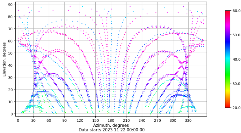
Azimuth-elevation plot for station TALV. Signal to Noise S1C Data file TALV00ESP_R_2023326.xtr
