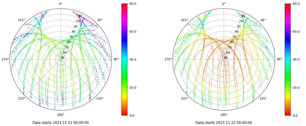
Skyplot for station TALV. Parameter M1C Data file TALV00ESP_R_2023326.xtr Skyplot for station TALV. Parameter M2P Data file TALV00ESP_R_2023326.xtr
