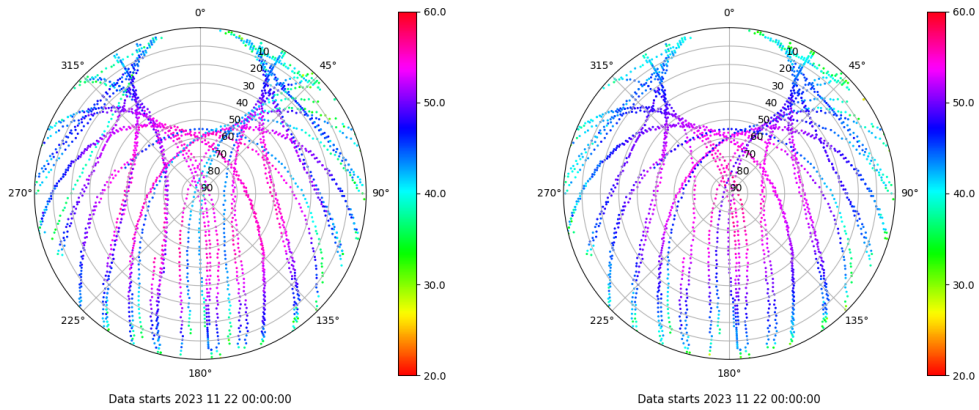
Skyplot for station TALV. Signal to Noise S1C Data file TALV00ESP_R_2023326.xtr Skyplot for station TALV. Signal to Noise S2P Data file TALV00ESP_R_2023326.xtr
