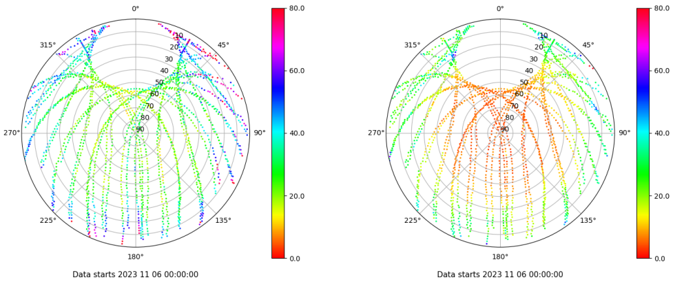
Skyplot for station TALV. Parameter M1C Data file TALV00ESP_R_2023310.xtr Skyplot for station TALV. Parameter M2P Data file TALV00ESP_R_2023310.xtr
