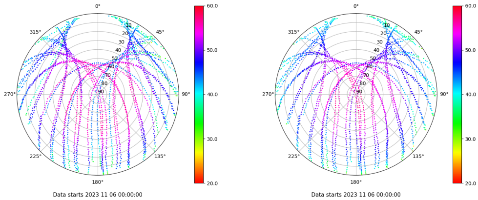
Skyplot for station TALV. Signal to Noise S1C Data file TALV00ESP_R_2023310.xtr Skyplot for station TALV. Signal to Noise S2P Data file TALV00ESP_R_2023310.xtr
