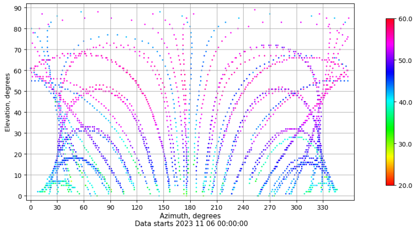
Azimuth-elevation plot for station TALV. Signal to Noise S1C Data file TALV00ESP_R_2023310.xtr
