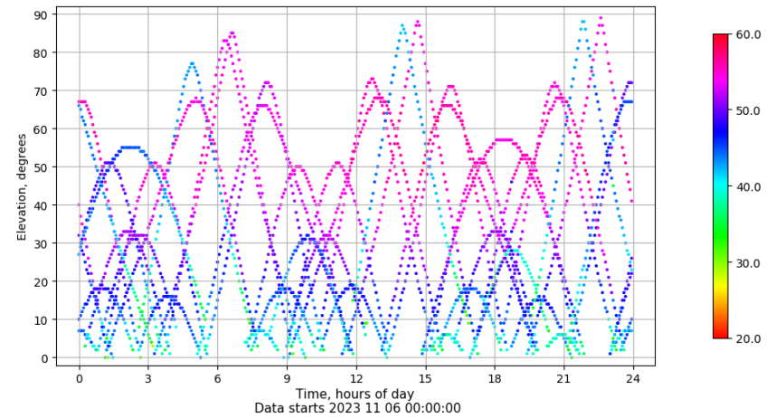
Time-elevation plot for station TALV. Signal to Noise S1C Data file TALV00ESP_R_2023310.xtr
