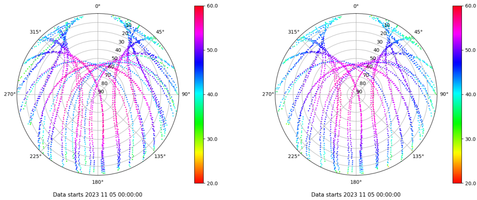
Skyplot for station TALV. Signal to Noise S1C Data file TALV00ESP_R_2023309.xtr Skyplot for station TALV. Signal to Noise S2P Data file TALV00ESP_R_2023309.xtr
