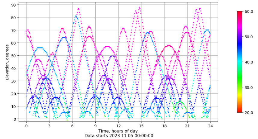
Time-elevation plot for station TALV. Signal to Noise S1C Data file TALV00ESP_R_2023309.xtr
