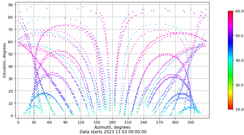
Azimuth-elevation plot for station TALV. Signal to Noise S1C Data file TALV00ESP_R_2023307.xtr
