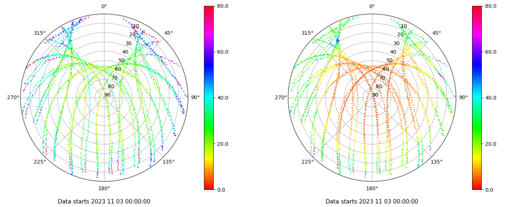
Skyplot for station TALV. Parameter M1C Data file TALV00ESP_R_2023307.xtr Skyplot for station TALV. Parameter M2P Data file TALV00ESP_R_2023307.xtr
