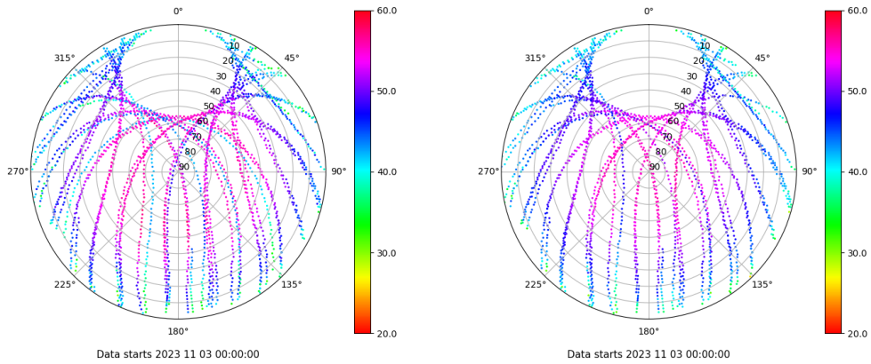
Skyplot for station TALV. Signal to Noise S1C Data file TALV00ESP_R_2023307.xtr Skyplot for station TALV. Signal to Noise S2P Data file TALV00ESP_R_2023307.xtr
