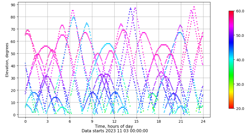
Time-elevation plot for station TALV. Signal to Noise S1C Data file TALV00ESP_R_2023307.xtr
