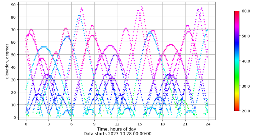
Time-elevation plot for station TALV. Signal to Noise S1C Data file TALV00ESP_R_2023301.xtr
