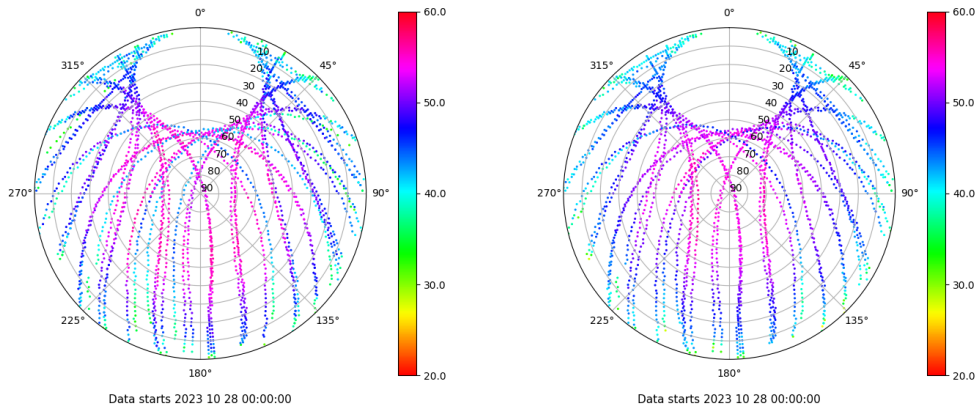
Skyplot for station TALV. Signal to Noise S1C Data file TALV00ESP_R_2023301.xtr Skyplot for station TALV. Signal to Noise S2P Data file TALV00ESP_R_2023301.xtr
