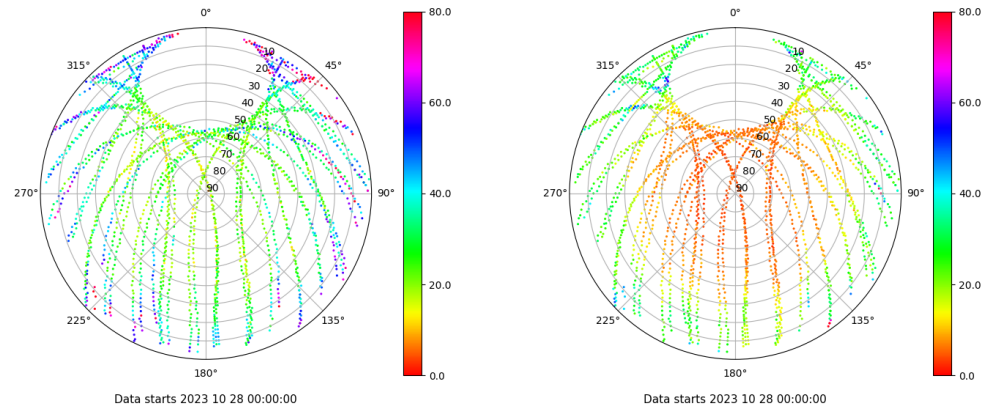
Skyplot for station TALV. Parameter M1C Data file TALV00ESP_R_2023301.xtr Skyplot for station TALV. Parameter M2P Data file TALV00ESP_R_2023301.xtr
