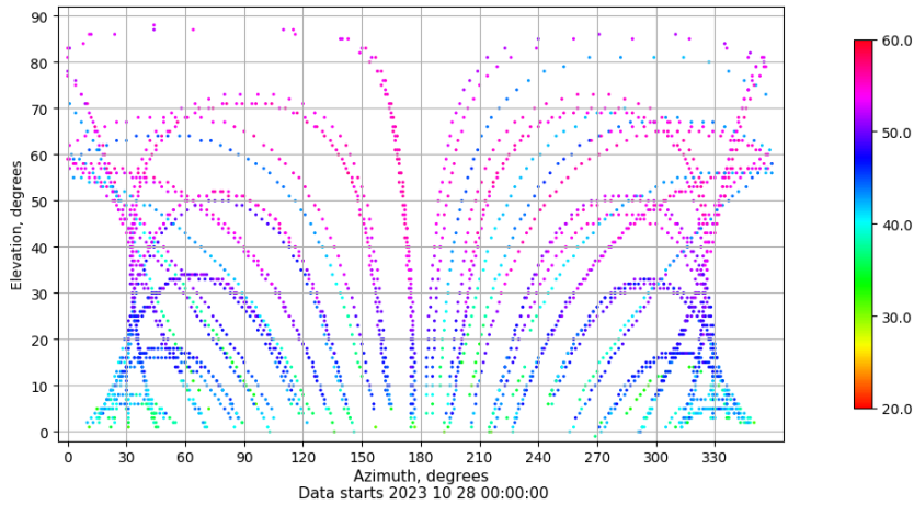
Azimuth-elevation plot for station TALV. Signal to Noise S1C Data file TALV00ESP_R_2023301.xtr
