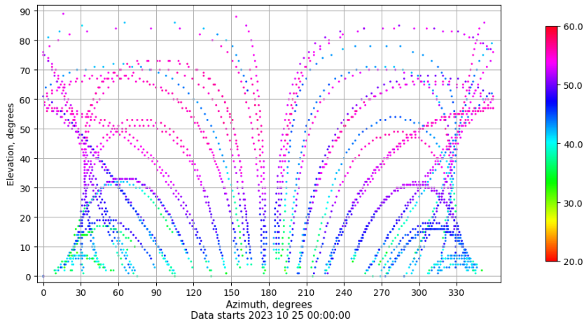
Azimuth-elevation plot for station TALV. Signal to Noise S1C Data file TALV00ESP_R_2023298.xtr
