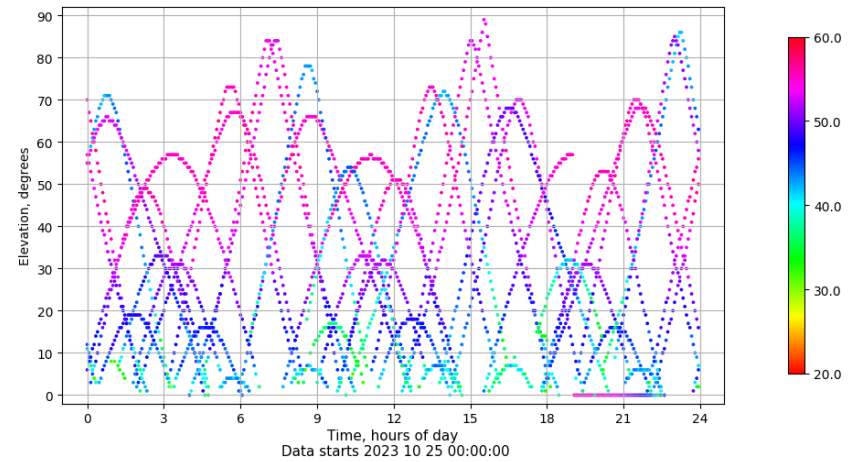
Time-elevation plot for station TALV. Signal to Noise S1C Data file TALV00ESP_R_2023298.xtr
