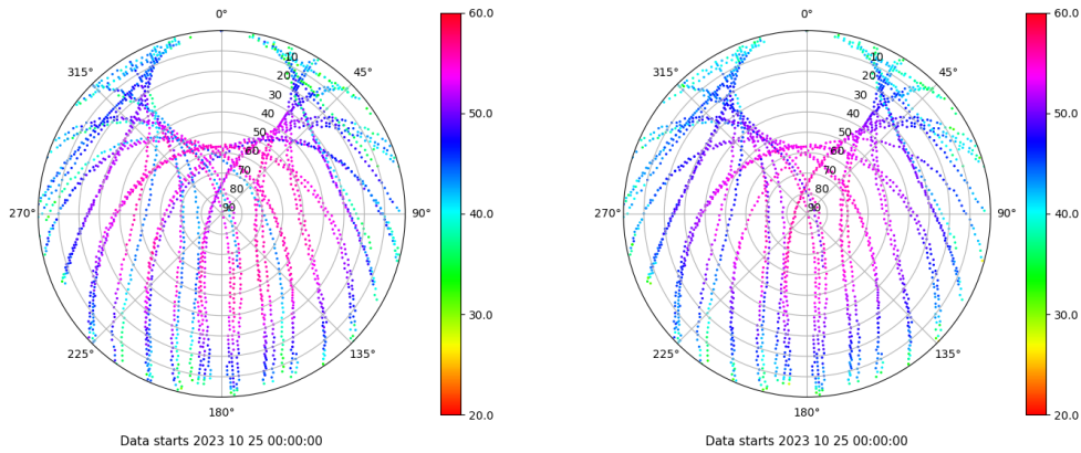
Skyplot for station TALV. Signal to Noise S1C Data file TALV00ESP_R_2023298.xtr Skyplot for station TALV. Signal to Noise S2P Data file TALV00ESP_R_2023298.xtr
