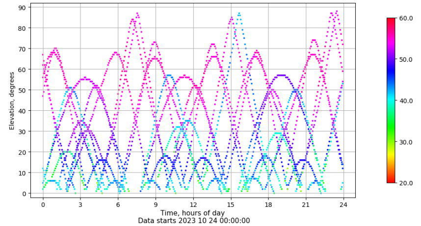
Time-elevation plot for station TALV. Signal to Noise S1C Data file TALV00ESP_R_2023297.xtr
