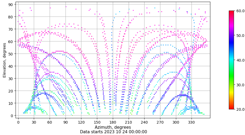
Azimuth-elevation plot for station TALV. Signal to Noise S1C Data file TALV00ESP_R_2023297.xtr
