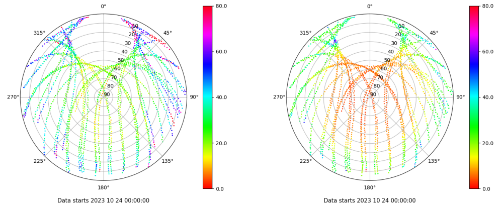
Skyplot for station TALV. Parameter M1C Data file TALV00ESP_R_2023297.xtr Skyplot for station TALV. Parameter M2P Data file TALV00ESP_R_2023297.xtr
