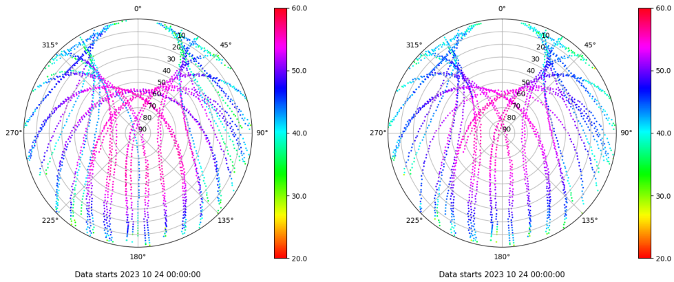
Skyplot for station TALV. Signal to Noise S1C Data file TALV00ESP_R_2023297.xtr Skyplot for station TALV. Signal to Noise S2P Data file TALV00ESP_R_2023297.xtr
