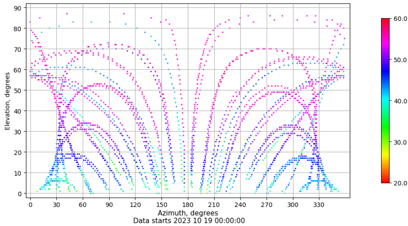
Azimuth-elevation plot for station TALV. Signal to Noise S1C Data file TALV00ESP_R_2023292.xtr
