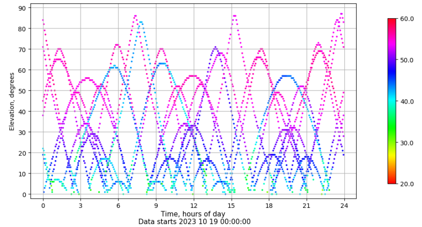
Time-elevation plot for station TALV. Signal to Noise S1C Data file TALV00ESP_R_2023292.xtr
