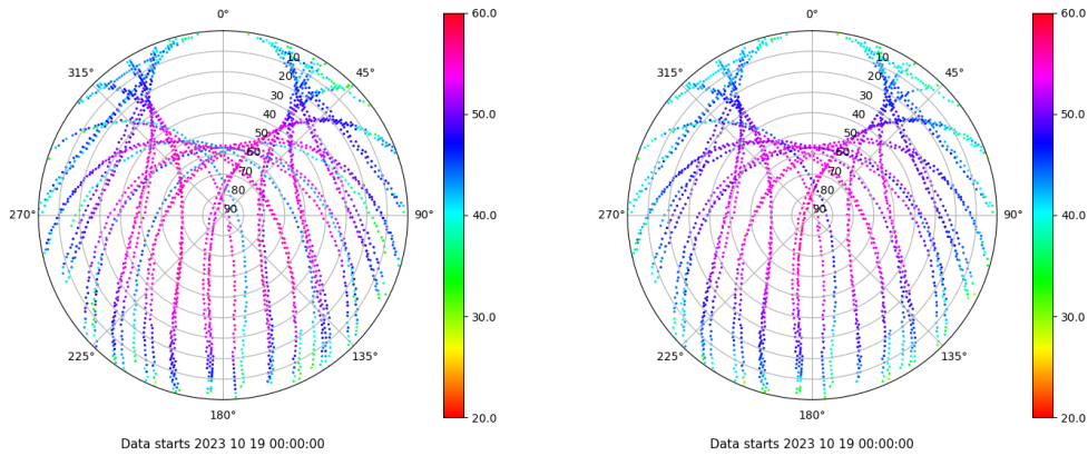
Skyplot for station TALV. Signal to Noise S1C Data file TALV00ESP_R_2023292.xtr Skyplot for station TALV. Signal to Noise S2P Data file TALV00ESP_R_2023292.xtr
