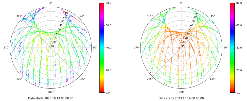
Skyplot for station TALV. Parameter M1C Data file TALV00ESP_R_2023292.xtr Skyplot for station TALV. Parameter M2P Data file TALV00ESP_R_2023292.xtr
