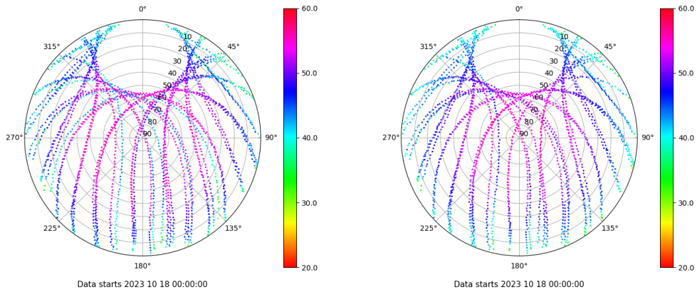
Skyplot for station TALV. Signal to Noise S1C Data file TALV00ESP_R_2023291.xtr Skyplot for station TALV. Signal to Noise S2P Data file TALV00ESP_R_2023291.xtr
