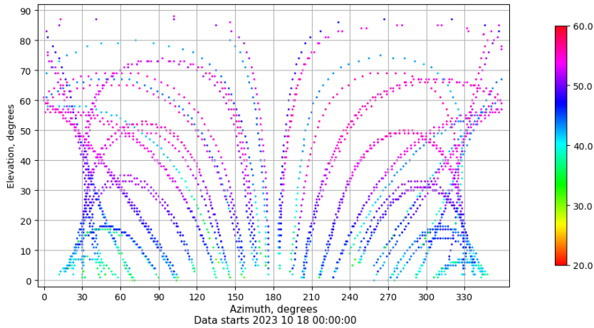
Azimuth-elevation plot for station TALV. Signal to Noise S1C Data file TALV00ESP_R_2023291.xtr
