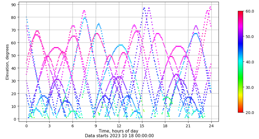
Time-elevation plot for station TALV. Signal to Noise S1C Data file TALV00ESP_R_2023291.xtr
