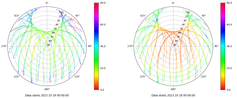
Skyplot for station TALV. Parameter M1C Data file TALV00ESP_R_2023291.xtr Skyplot for station TALV. Parameter M2P Data file TALV00ESP_R_2023291.xtr
