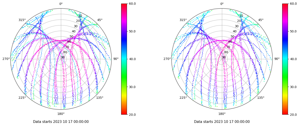
Skyplot for station TALV. Signal to Noise S1C Data file TALV00ESP_R_2023290.xtr Skyplot for station TALV. Signal to Noise S2P Data file TALV00ESP_R_2023290.xtr
