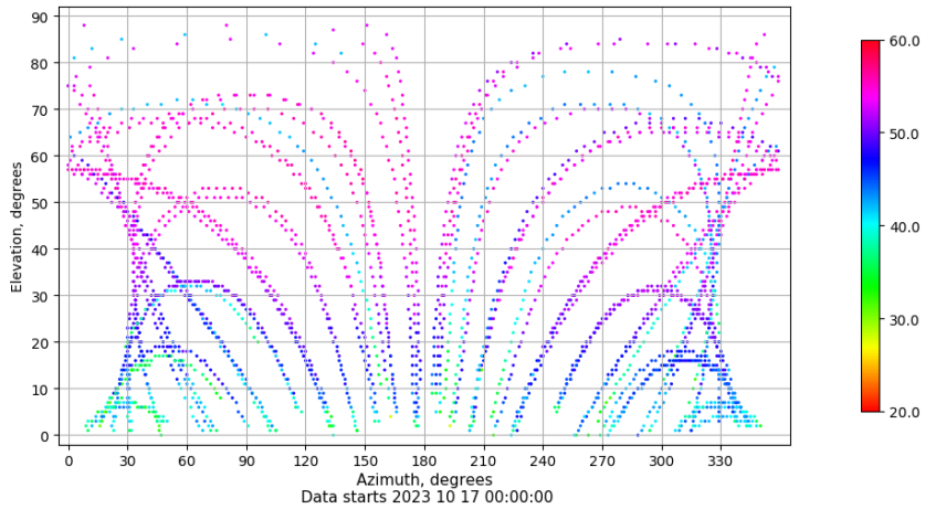
Azimuth-elevation plot for station TALV. Signal to Noise S1C Data file TALV00ESP_R_2023290.xtr
