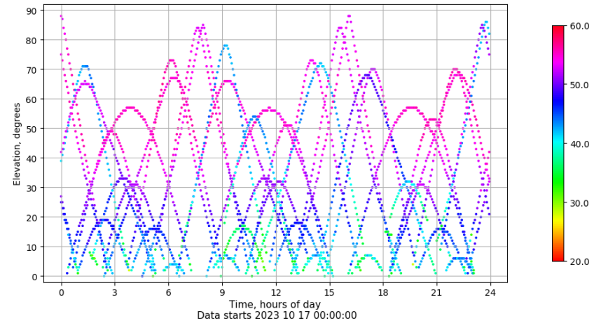
Time-elevation plot for station TALV. Signal to Noise S1C Data file TALV00ESP_R_2023290.xtr
