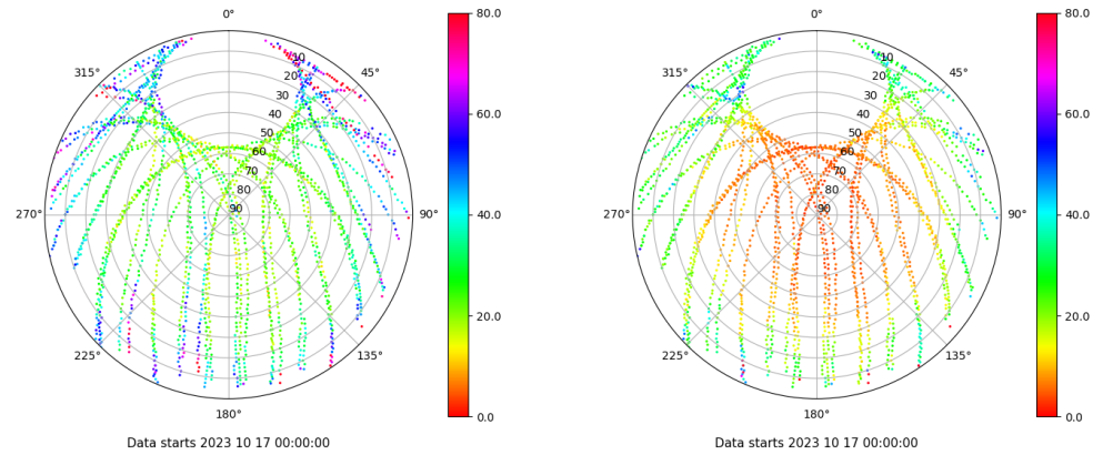
Skyplot for station TALV. Parameter M1C Data file TALV00ESP_R_2023290.xtr Skyplot for station TALV. Parameter M2P Data file TALV00ESP_R_2023290.xtr
