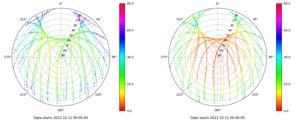
Skyplot for station TALV. Parameter M1C Data file TALV00ESP_R_2023284.xtr Skyplot for station TALV. Parameter M2P Data file TALV00ESP_R_2023284.xtr
