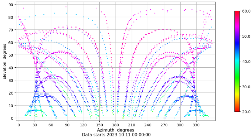
Azimuth-elevation plot for station TALV. Signal to Noise S1C Data file TALV00ESP_R_2023284.xtr
