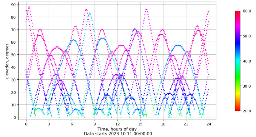
Time-elevation plot for station TALV. Signal to Noise S1C Data file TALV00ESP_R_2023284.xtr
