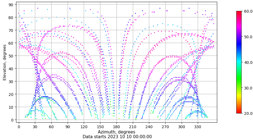
Azimuth-elevation plot for station TALV. Signal to Noise S1C Data file TALV00ESP_R_2023283.xtr
