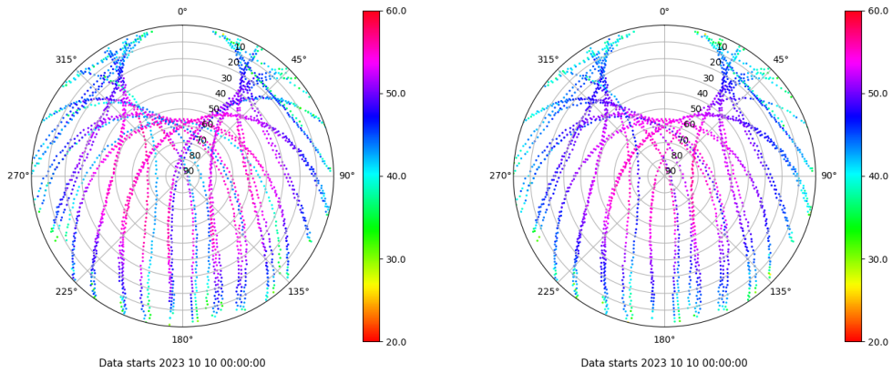
Skyplot for station TALV. Signal to Noise S1C Data file TALV00ESP_R_2023283.xtr Skyplot for station TALV. Signal to Noise S2P Data file TALV00ESP_R_2023283.xtr
