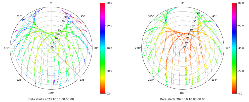
Skyplot for station TALV. Parameter M1C Data file TALV00ESP_R_2023283.xtr Skyplot for station TALV. Parameter M2P Data file TALV00ESP_R_2023283.xtr
