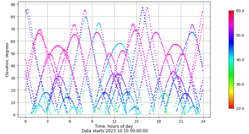
Time-elevation plot for station TALV. Signal to Noise S1C Data file TALV00ESP_R_2023283.xtr
