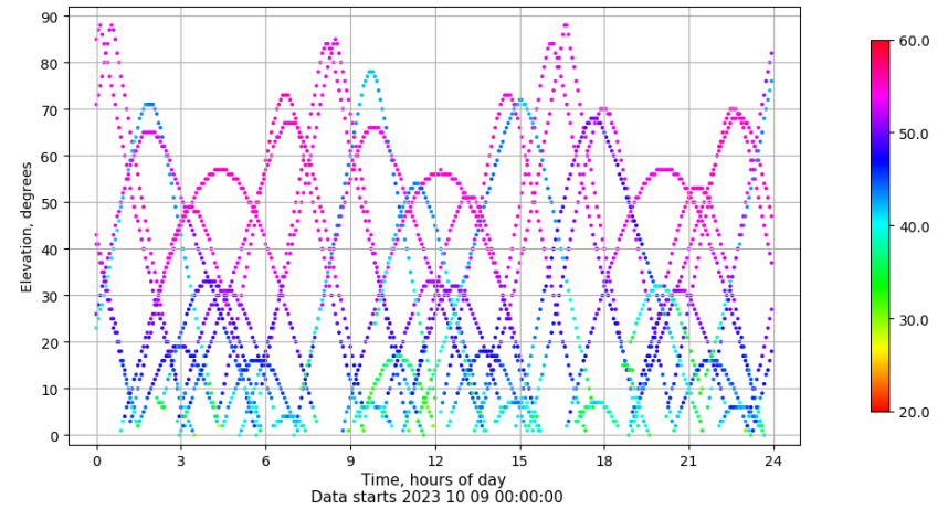
Time-elevation plot for station TALV. Signal to Noise S1C Data file TALV00ESP_R_2023282.xtr
