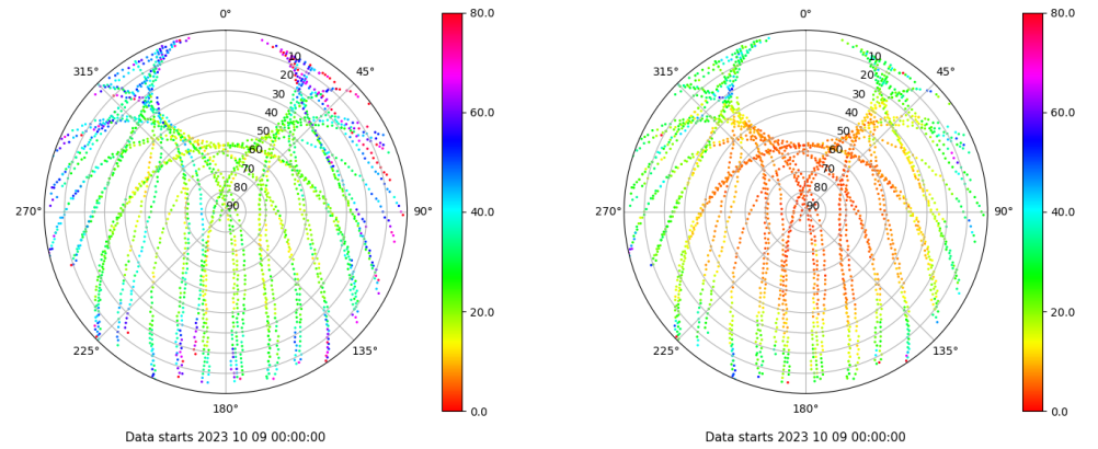
Skyplot for station TALV. Parameter M1C Data file TALV00ESP_R_2023282.xtr Skyplot for station TALV. Parameter M2P Data file TALV00ESP_R_2023282.xtr
