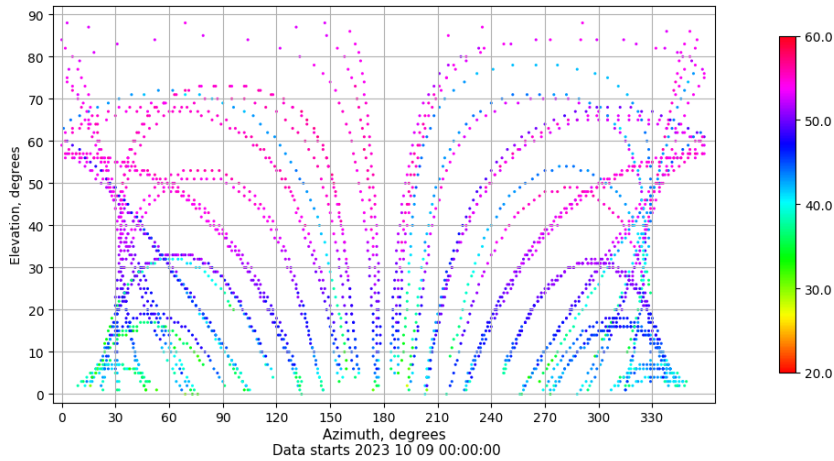
Azimuth-elevation plot for station TALV. Signal to Noise S1C Data file TALV00ESP_R_2023282.xtr
