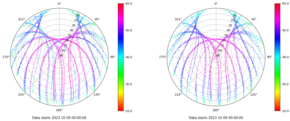
Skyplot for station TALV. Signal to Noise S1C Data file TALV00ESP_R_2023282.xtr Skyplot for station TALV. Signal to Noise S2P Data file TALV00ESP_R_2023282.xtr
