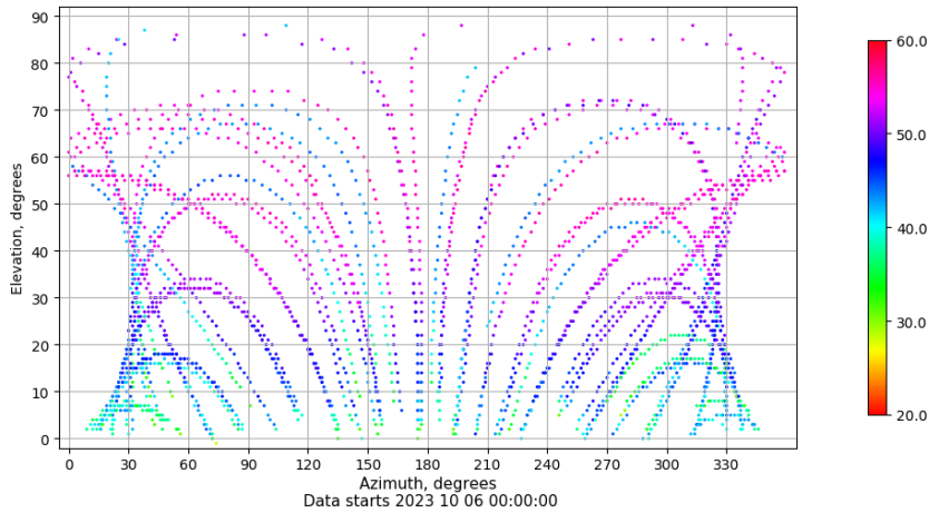
Azimuth-elevation plot for station TALV. Signal to Noise S1C Data file TALV00ESP_R_2023279.xtr
