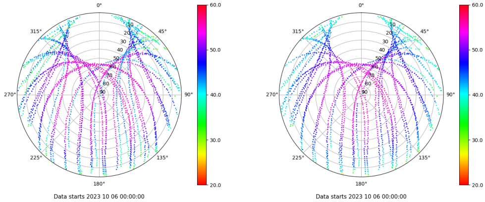
Skyplot for station TALV. Signal to Noise S1C Data file TALV00ESP_R_2023279.xtr Skyplot for station TALV. Signal to Noise S2P Data file TALV00ESP_R_2023279.xtr
