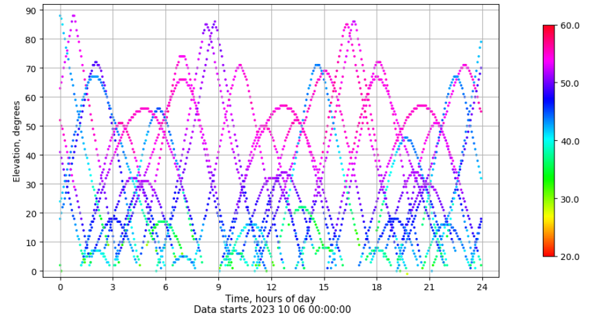
Time-elevation plot for station TALV. Signal to Noise S1C Data file TALV00ESP_R_2023279.xtr
