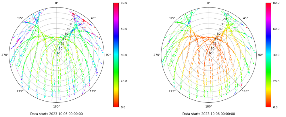
Skyplot for station TALV. Parameter M1C Data file TALV00ESP_R_2023279.xtr Skyplot for station TALV. Parameter M2P Data file TALV00ESP_R_2023279.xtr
