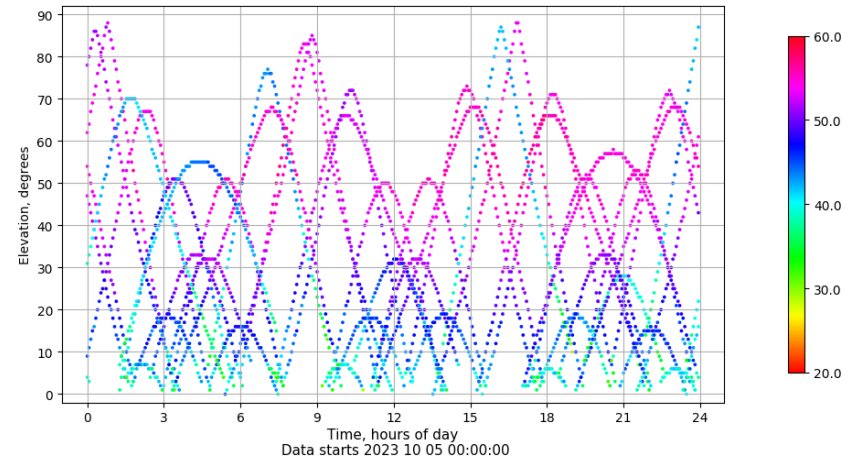
Time-elevation plot for station TALV. Signal to Noise S1C Data file TALV00ESP_R_2023278.xtr
