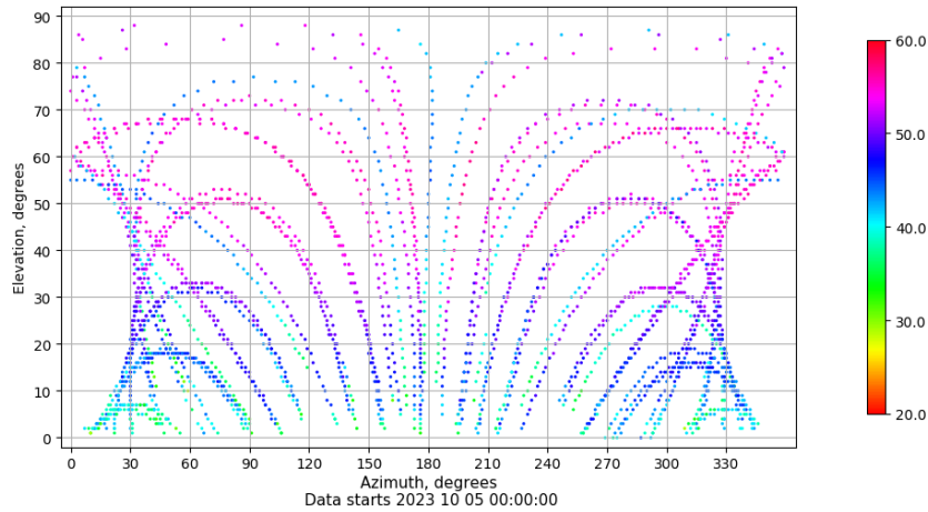
Azimuth-elevation plot for station TALV. Signal to Noise S1C Data file TALV00ESP_R_2023278.xtr
