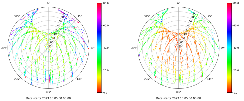
Skyplot for station TALV. Parameter M1C Data file TALV00ESP_R_2023278.xtr Skyplot for station TALV. Parameter M2P Data file TALV00ESP_R_2023278.xtr
