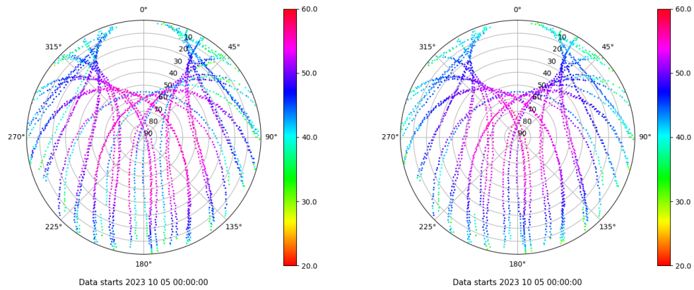
Skyplot for station TALV. Signal to Noise S1C Data file TALV00ESP_R_2023278.xtr Skyplot for station TALV. Signal to Noise S2P Data file TALV00ESP_R_2023278.xtr
