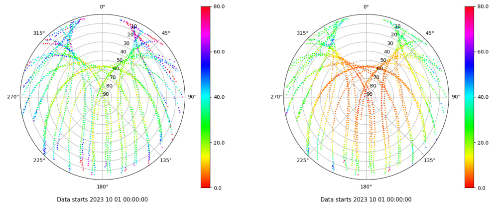
Skyplot for station TALV. Parameter M1C Data file TALV00ESP_R_2023274.xtr Skyplot for station TALV. Parameter M2P Data file TALV00ESP_R_2023274.xtr
