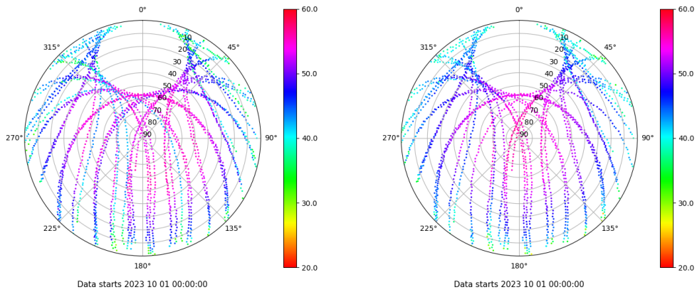
Skyplot for station TALV. Signal to Noise S1C Data file TALV00ESP_R_2023274.xtr Skyplot for station TALV. Signal to Noise S2P Data file TALV00ESP_R_2023274.xtr
