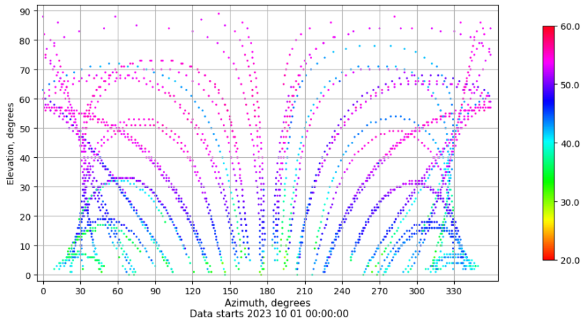
Azimuth-elevation plot for station TALV. Signal to Noise S1C Data file TALV00ESP_R_2023274.xtr
