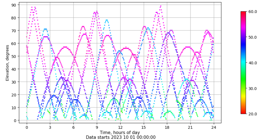
Time-elevation plot for station TALV. Signal to Noise S1C Data file TALV00ESP_R_2023274.xtr
