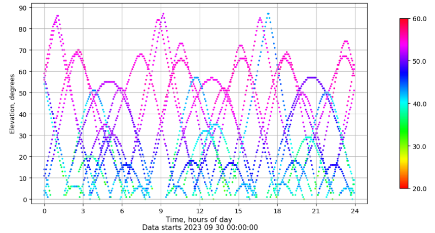
Time-elevation plot for station TALV. Signal to Noise S1C Data file TALV00ESP_R_2023273.xtr
