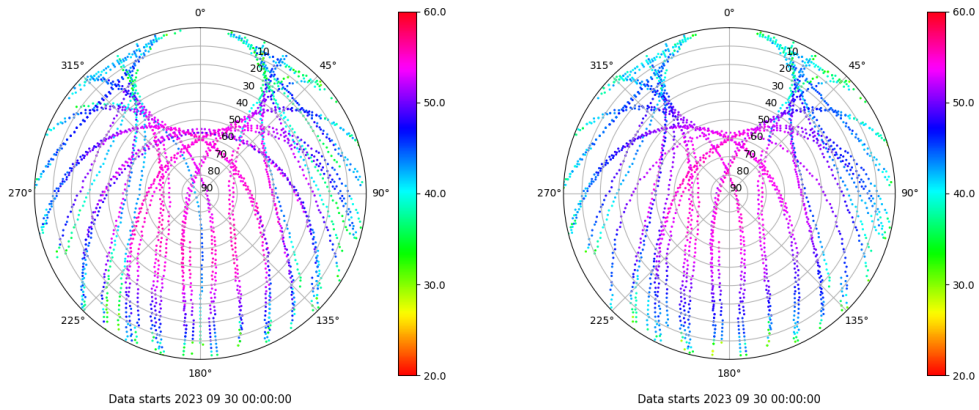
Skyplot for station TALV. Signal to Noise S1C Data file TALV00ESP_R_2023273.xtr Skyplot for station TALV. Signal to Noise S2P Data file TALV00ESP_R_2023273.xtr
