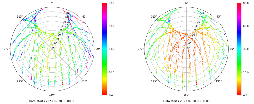
Skyplot for station TALV. Parameter M1C Data file TALV00ESP_R_2023273.xtr Skyplot for station TALV. Parameter M2P Data file TALV00ESP_R_2023273.xtr
