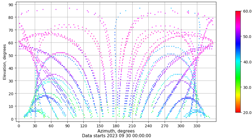
Azimuth-elevation plot for station TALV. Signal to Noise S1C Data file TALV00ESP_R_2023273.xtr
