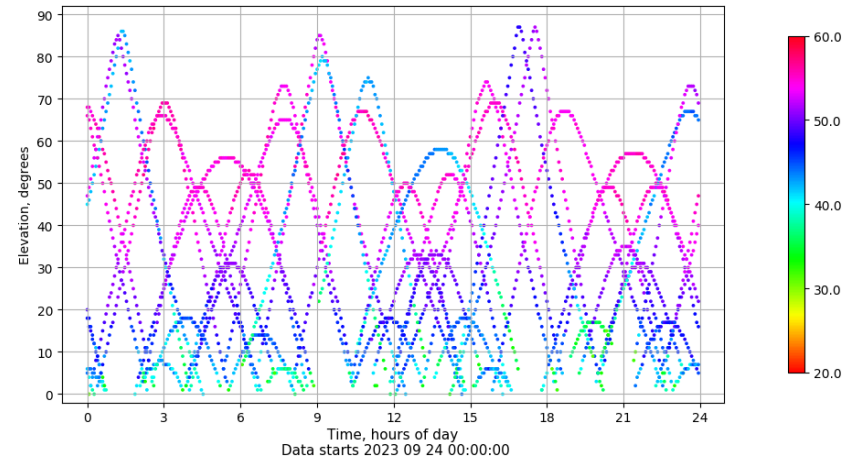
Time-elevation plot for station TALV. Signal to Noise S1C Data file TALV00ESP_R_2023267.xtr
