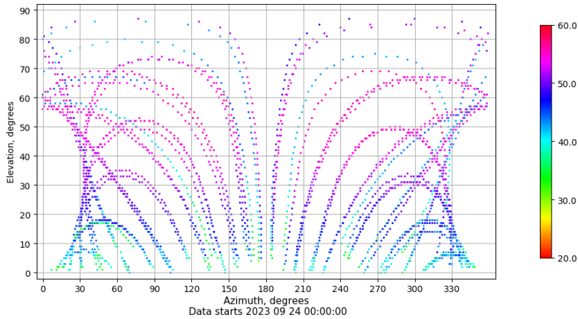
Azimuth-elevation plot for station TALV. Signal to Noise S1C Data file TALV00ESP_R_2023267.xtr
