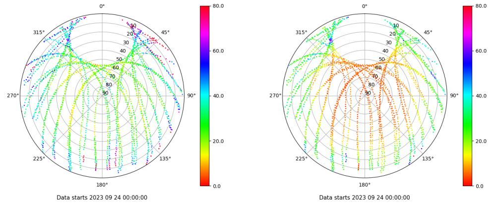
Skyplot for station TALV. Parameter M1C Data file TALV00ESP_R_2023267.xtr Skyplot for station TALV. Parameter M2P Data file TALV00ESP_R_2023267.xtr
