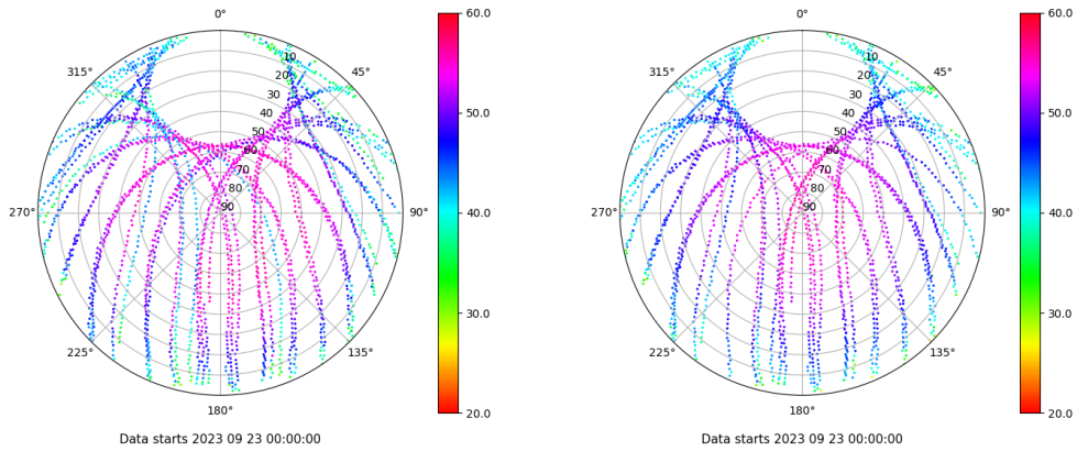
Skyplot for station TALV. Signal to Noise S1C Data file TALV00ESP_R_2023266.xtr Skyplot for station TALV. Signal to Noise S2P Data file TALV00ESP_R_2023266.xtr
