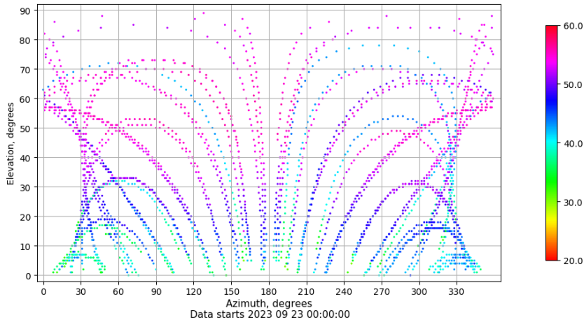
Azimuth-elevation plot for station TALV. Signal to Noise S1C Data file TALV00ESP_R_2023266.xtr
