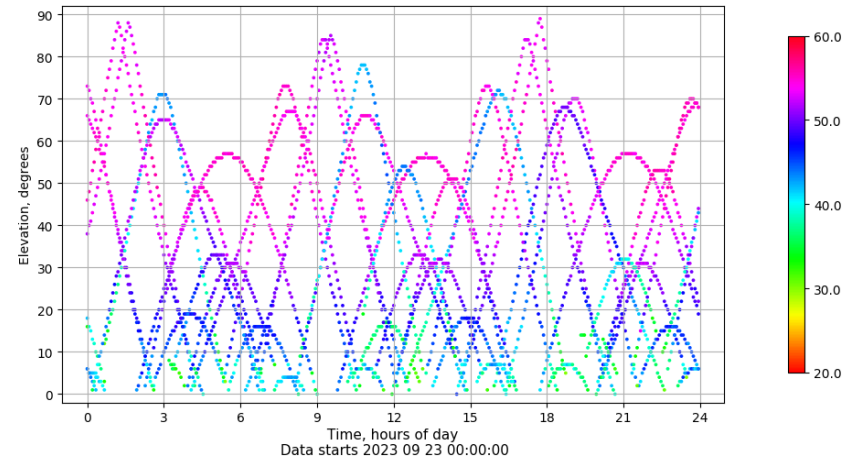
Time-elevation plot for station TALV. Signal to Noise S1C Data file TALV00ESP_R_2023266.xtr
