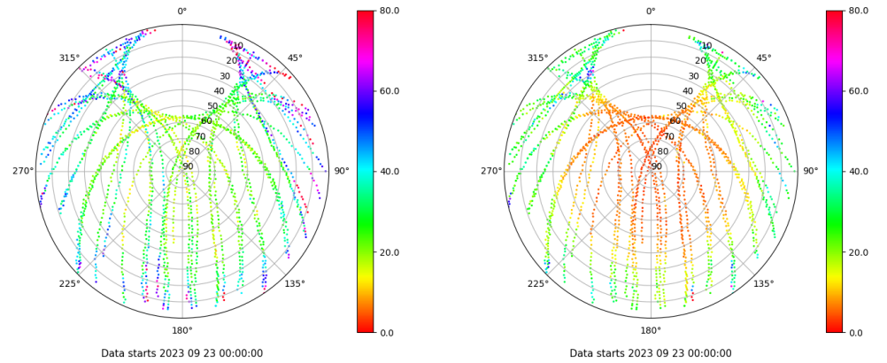
Skyplot for station TALV. Parameter M1C Data file TALV00ESP_R_2023266.xtr Skyplot for station TALV. Parameter M2P Data file TALV00ESP_R_2023266.xtr
