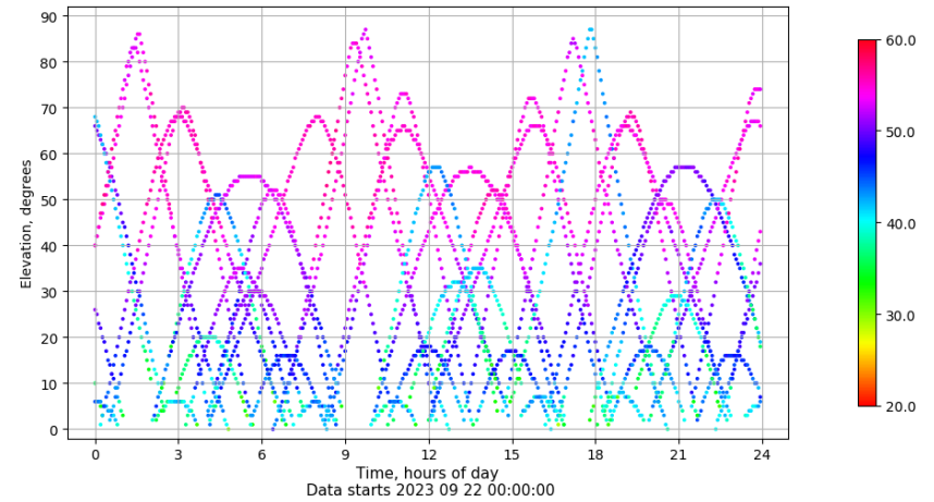
Time-elevation plot for station TALV. Signal to Noise S1C Data file TALV00ESP_R_2023265.xtr
