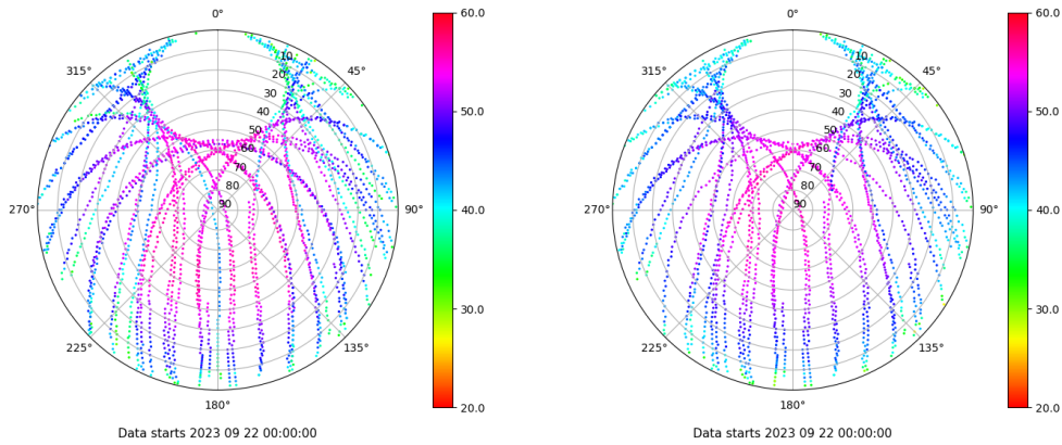
Skyplot for station TALV. Signal to Noise S1C Data file TALV00ESP_R_2023265.xtr Skyplot for station TALV. Signal to Noise S2P Data file TALV00ESP_R_2023265.xtr
