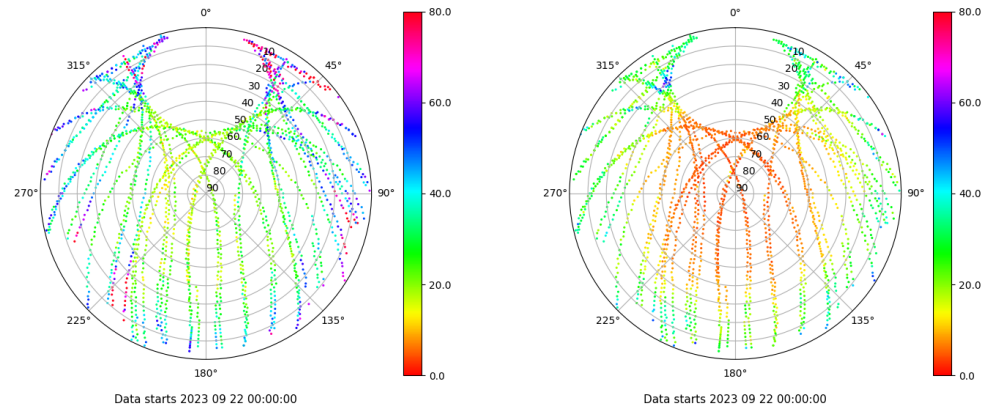
Skyplot for station TALV. Parameter M1C Data file TALV00ESP_R_2023265.xtr Skyplot for station TALV. Parameter M2P Data file TALV00ESP_R_2023265.xtr
