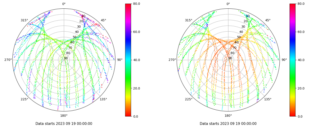
Skyplot for station TALV. Parameter M1C Data file TALV00ESP_R_2023262.xtr Skyplot for station TALV. Parameter M2P Data file TALV00ESP_R_2023262.xtr
