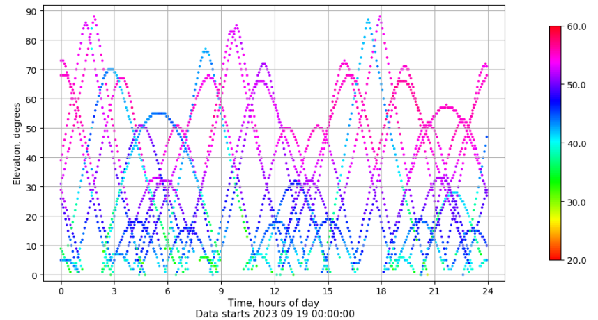
Time-elevation plot for station TALV. Signal to Noise S1C Data file TALV00ESP_R_2023262.xtr
