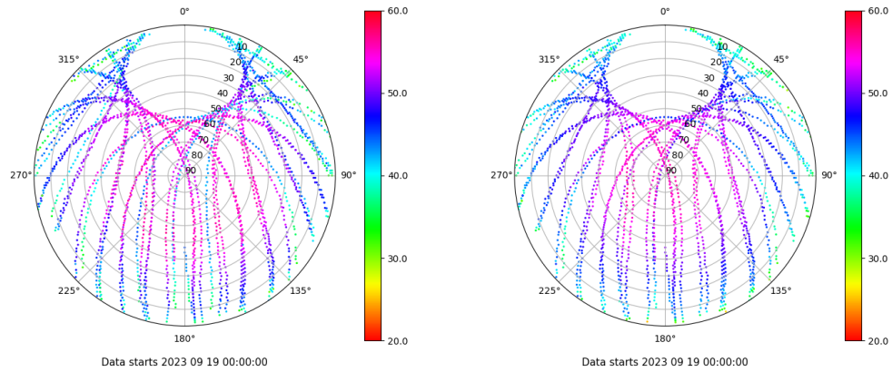
Skyplot for station TALV. Signal to Noise S1C Data file TALV00ESP_R_2023262.xtr Skyplot for station TALV. Signal to Noise S2P Data file TALV00ESP_R_2023262.xtr
