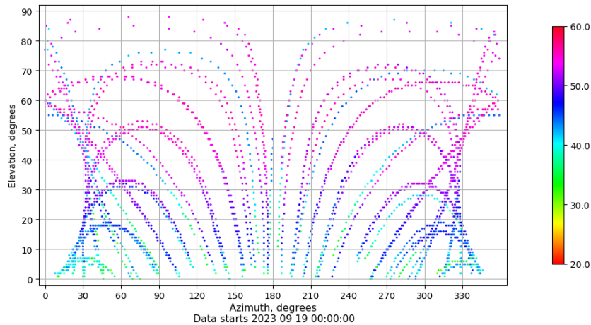
Azimuth-elevation plot for station TALV. Signal to Noise S1C Data file TALV00ESP_R_2023262.xtr
