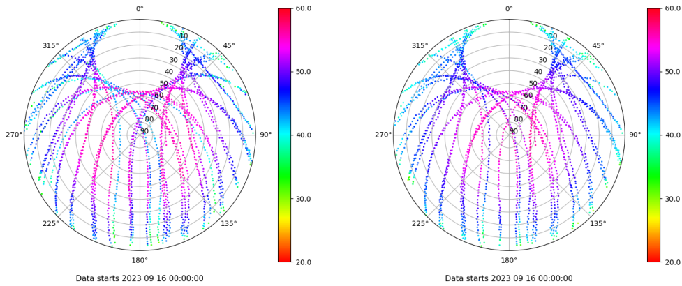
Skyplot for station TALV. Signal to Noise S1C Data file TALV00ESP_R_2023259.xtr Skyplot for station TALV. Signal to Noise S2P Data file TALV00ESP_R_2023259.xtr
