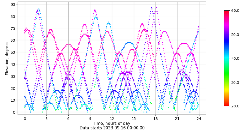
Time-elevation plot for station TALV. Signal to Noise S1C Data file TALV00ESP_R_2023259.xtr
