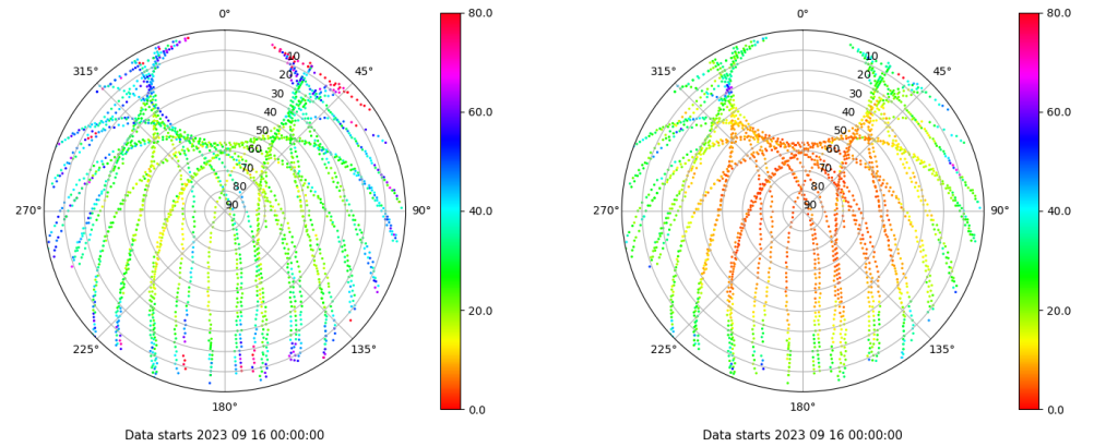
Skyplot for station TALV. Parameter M1C Data file TALV00ESP_R_2023259.xtr Skyplot for station TALV. Parameter M2P Data file TALV00ESP_R_2023259.xtr
