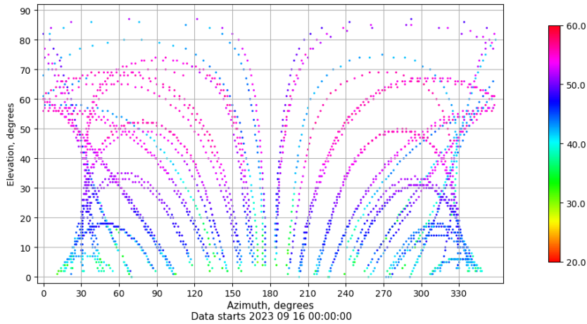
Azimuth-elevation plot for station TALV. Signal to Noise S1C Data file TALV00ESP_R_2023259.xtr
